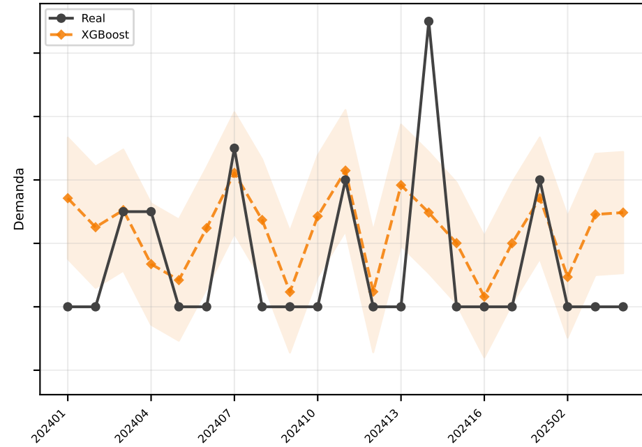
XGBoost MAE=1.9
