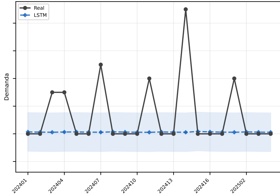
LSTM MAE=1.4
