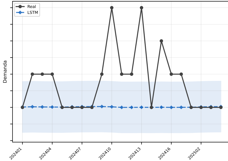
LSTM MAE=0.8
