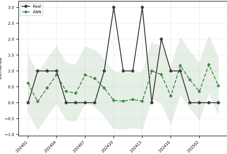
ANN MAE=0.9
