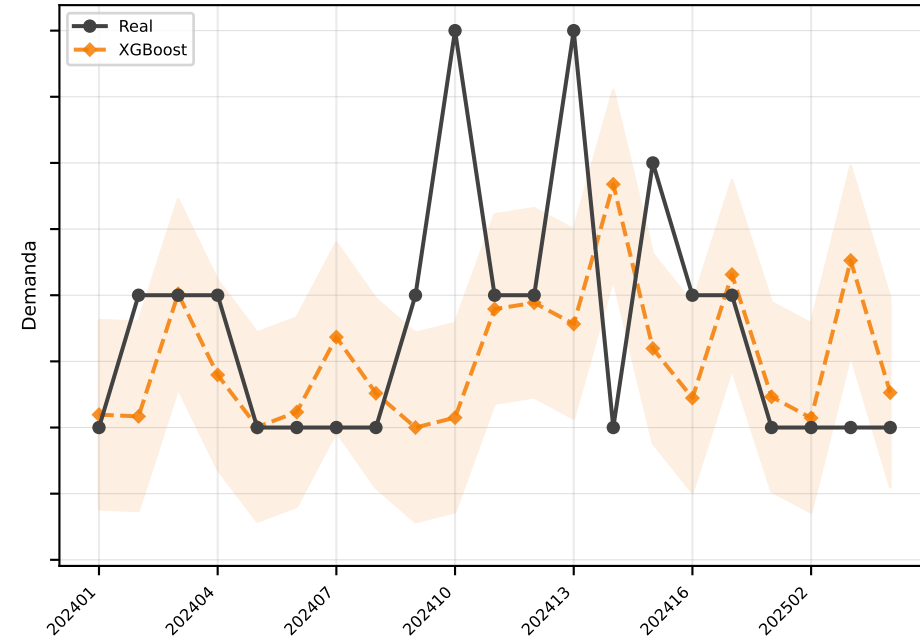
XGBoost MAE=0.7
