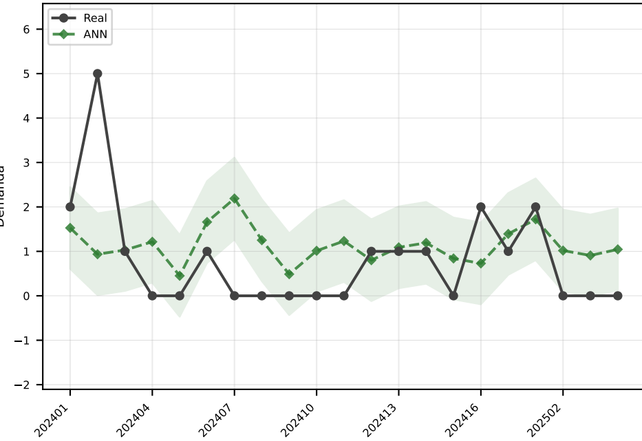
ANN MAE=0.9
