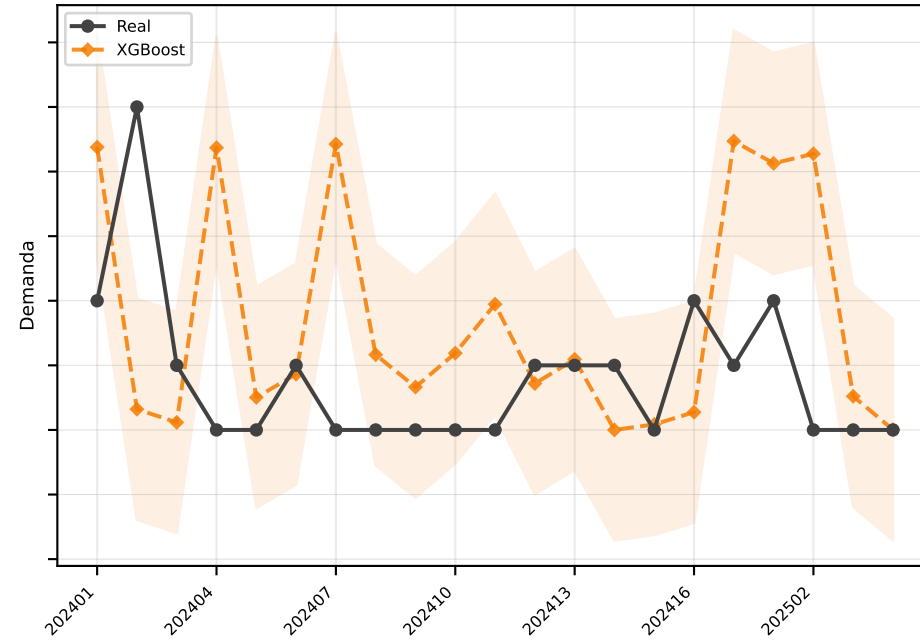
XGBoost MAE=1.7
