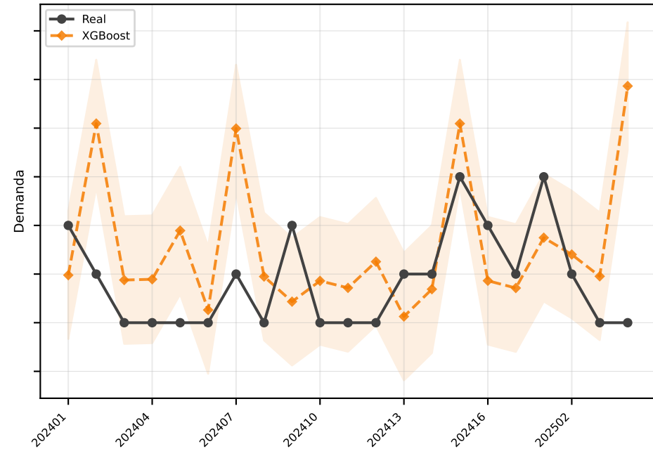
XGBoost MAE=1.3
