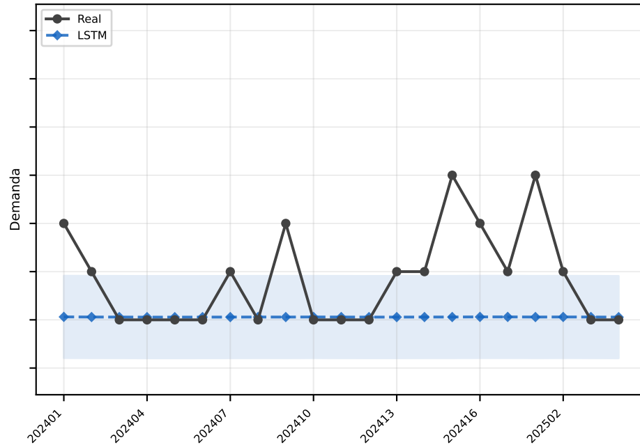
LSTM MAE=0.9
