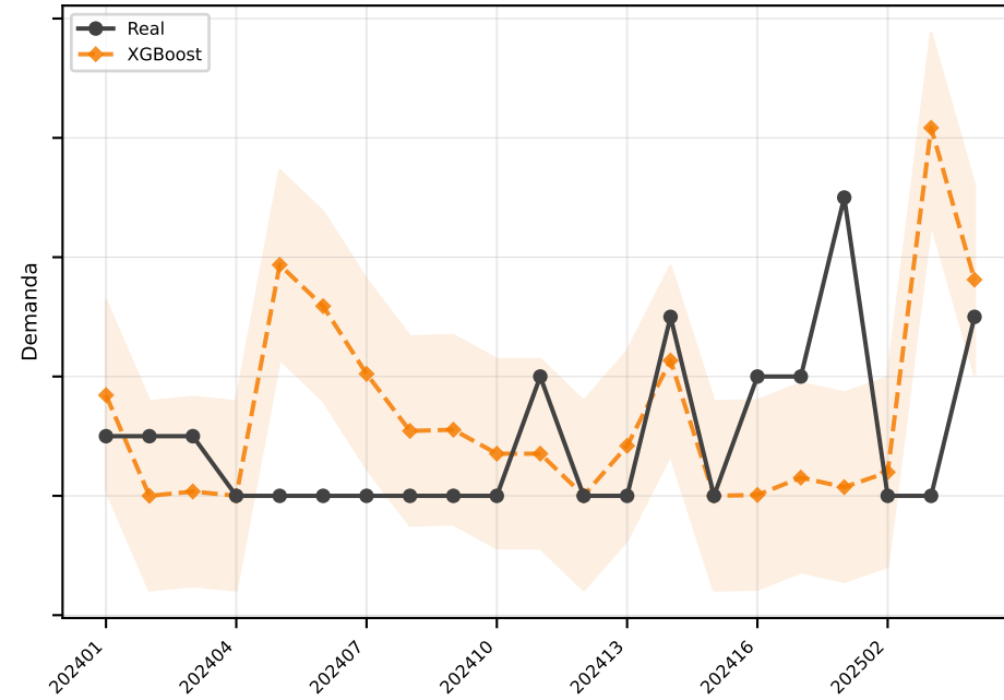
XGBoost MAE=1.6
