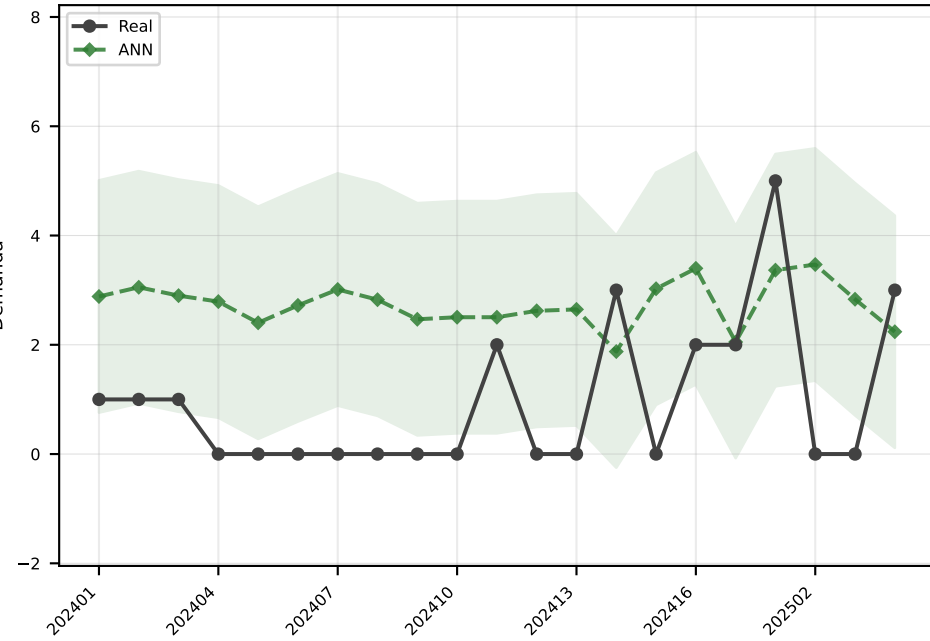
ANN MAE=2.1
