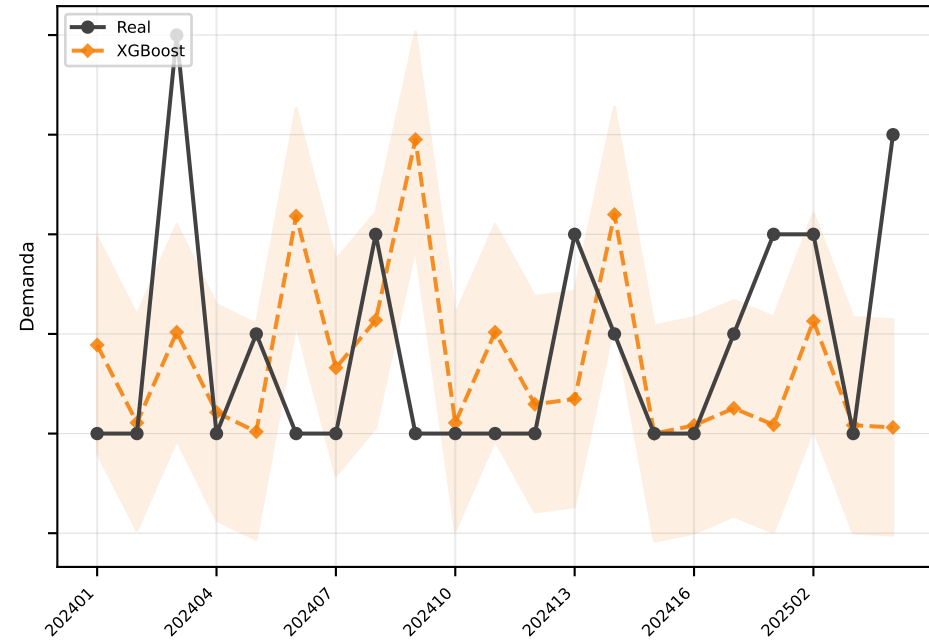
XGBoost MAE=1.1
