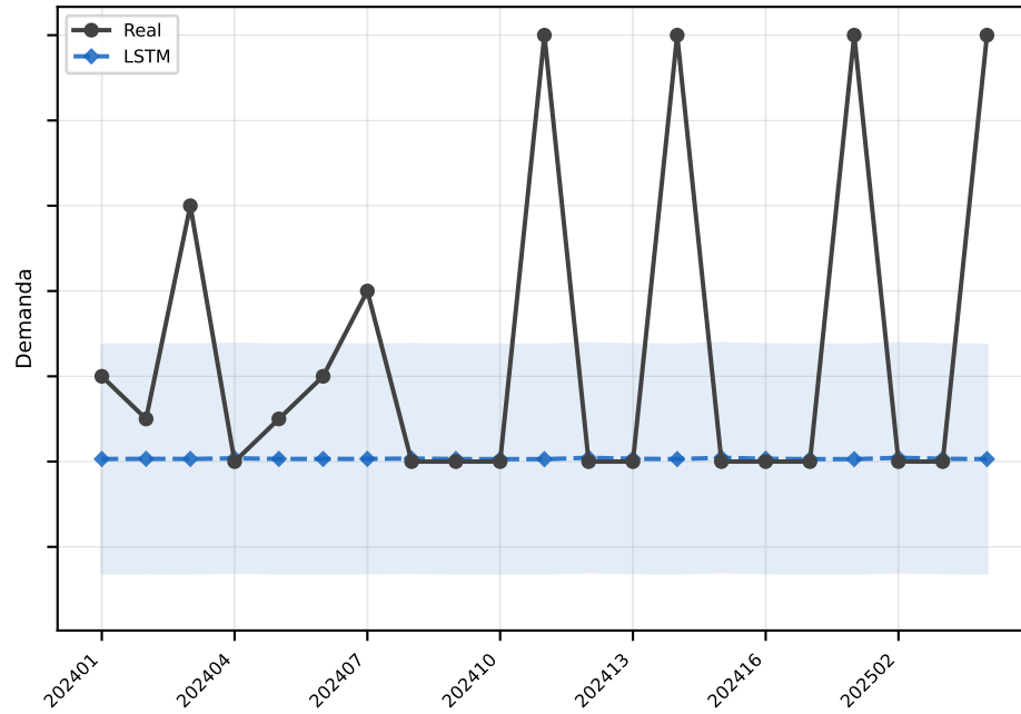
LSTM MAE=2.7
