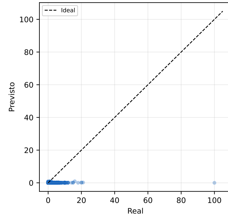
LSTM (n=3,045)
