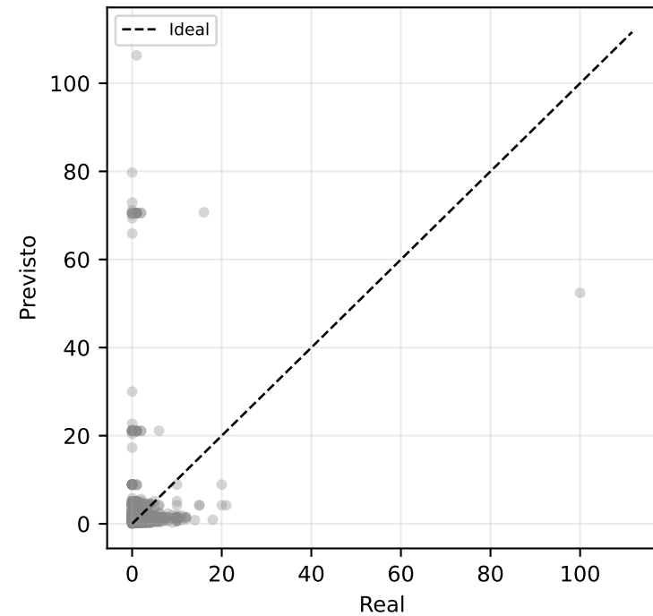
ARIMA (n=3,045)
