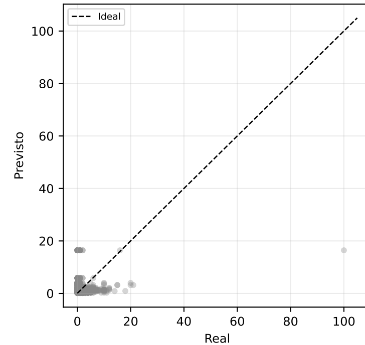
Croston (n=3,045)
