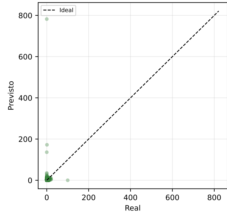
ANN (n=3,045)
