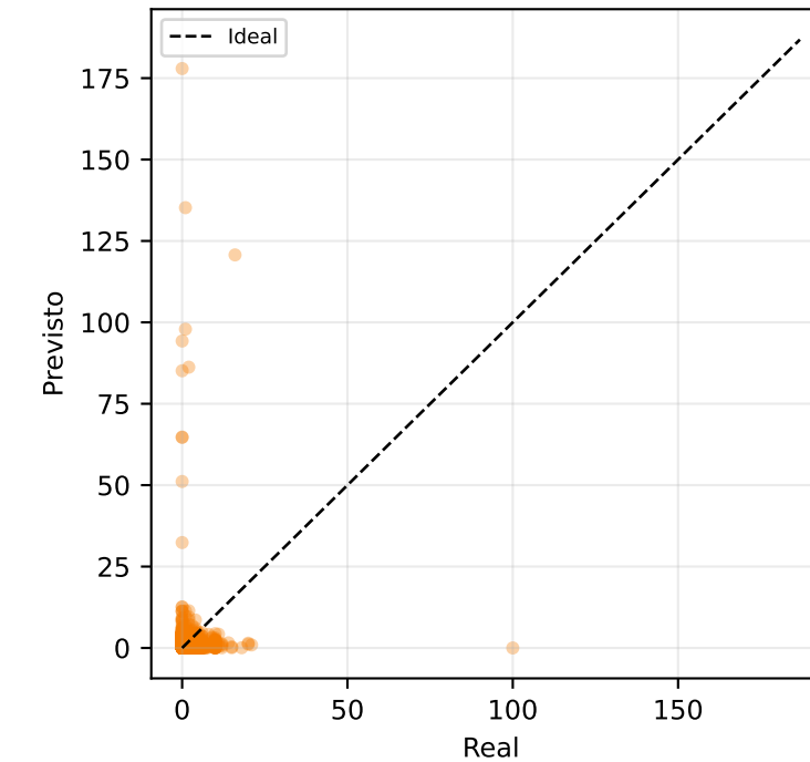
XGBoost (n=3,045)
