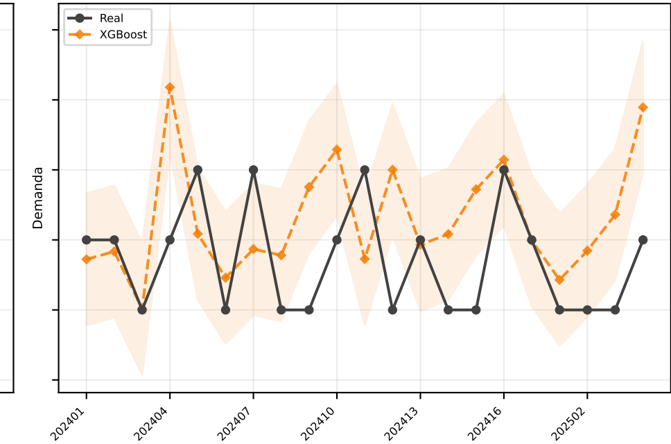
XGBoost MAE=0.9
