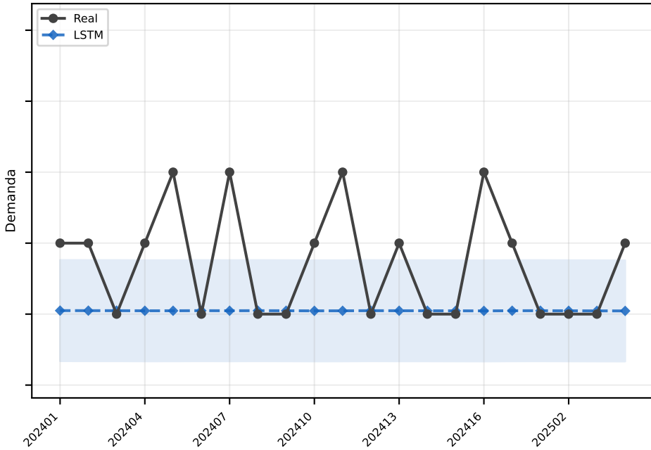
LSTM MAE=0.7
