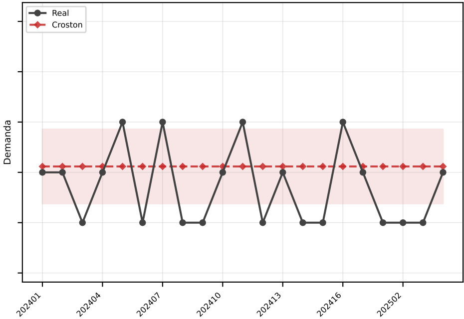
Croston MAE=0.7
