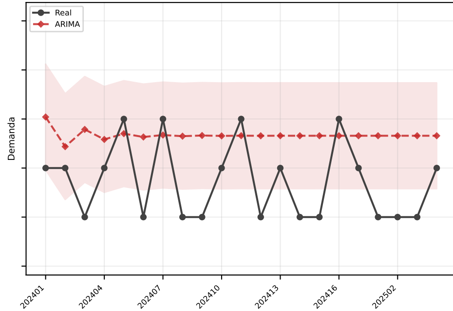
ARIMA MAE=1.1
