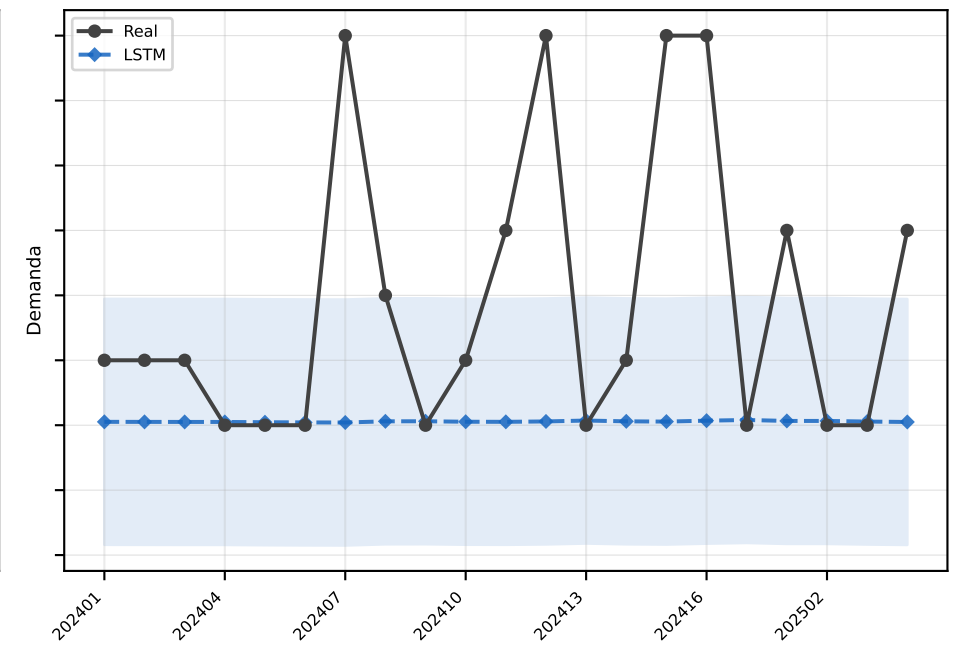
LSTM MAE=1.9
