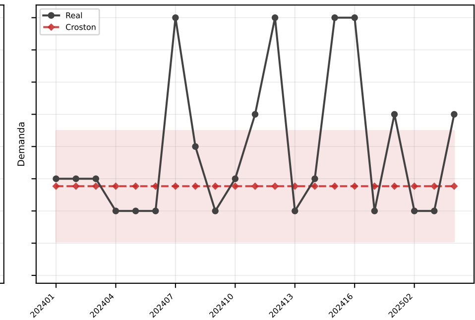
Croston MAE=1.7
