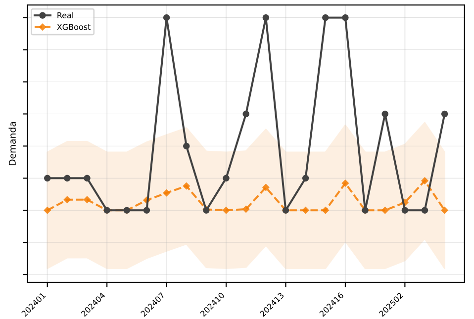
XGBoost MAE=1.8
