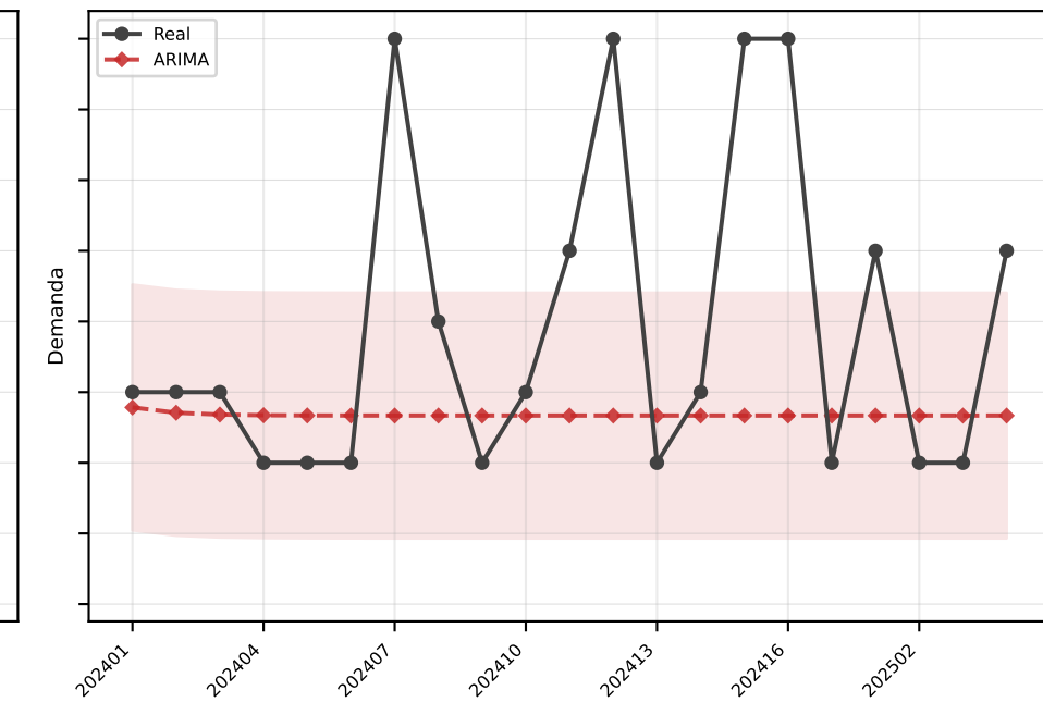
ARIMA MAE=1.7
