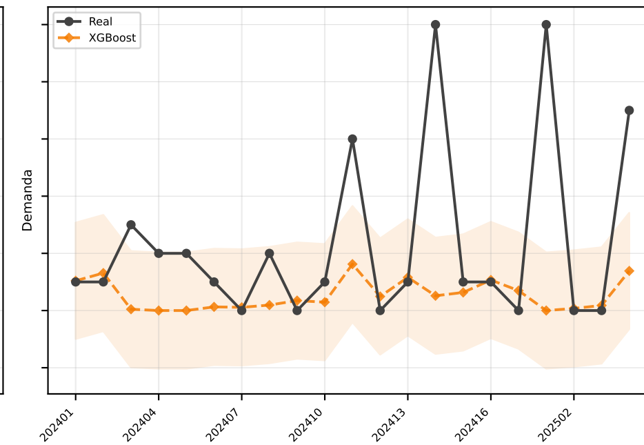
XGBoost MAE=2.0
