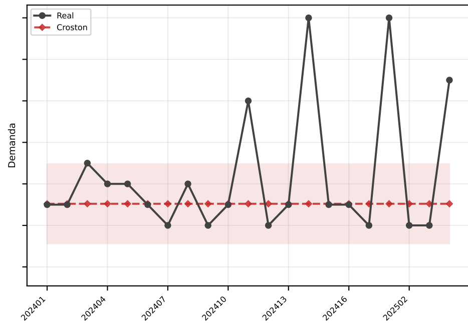
Croston MAE=1.9
