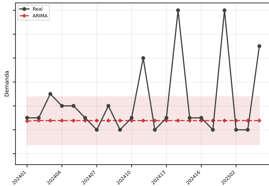
ARIMA MAE=2.0
