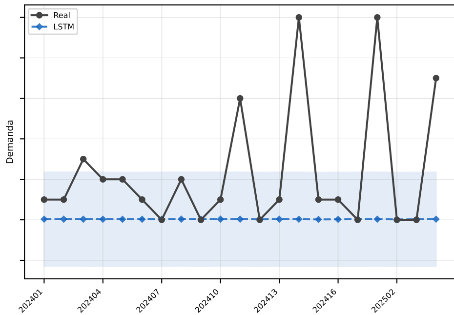
LSTM MAE=2.3
