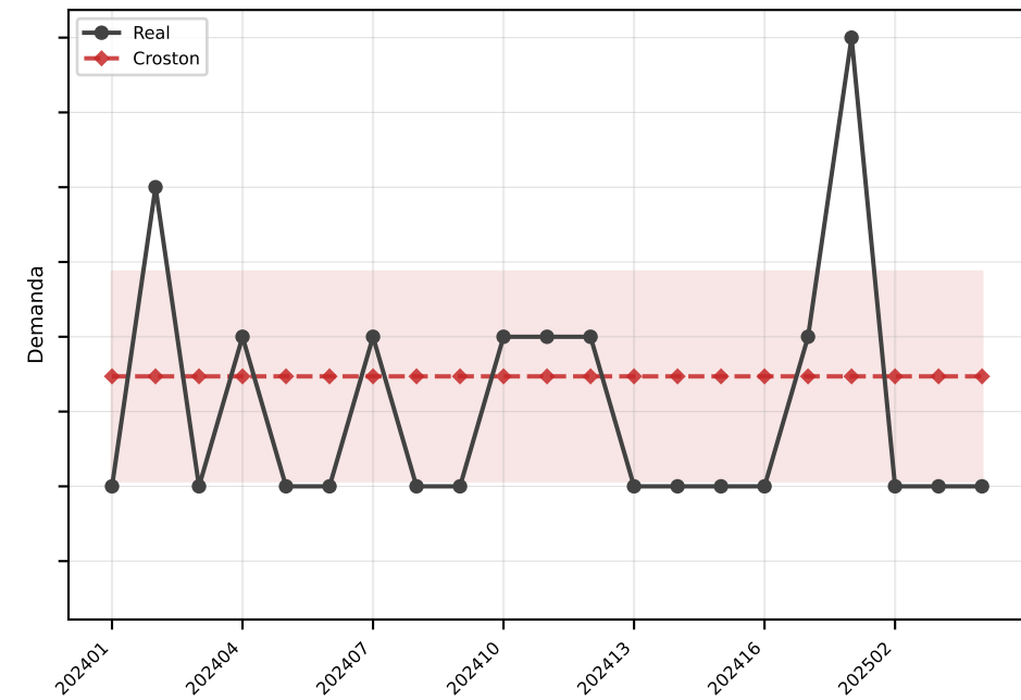
Croston MAE=0.7
