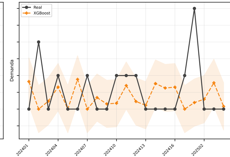
XGBoost MAE=0.7
