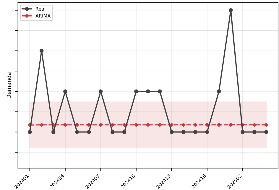
ARIMA MAE=0.6
