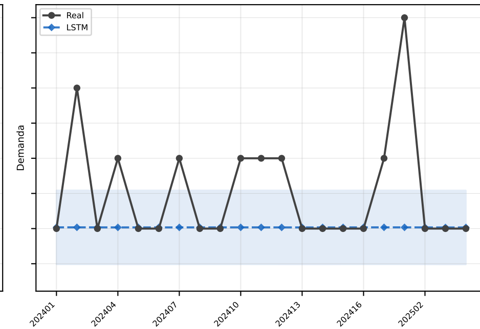
LSTM MAE=0.5
