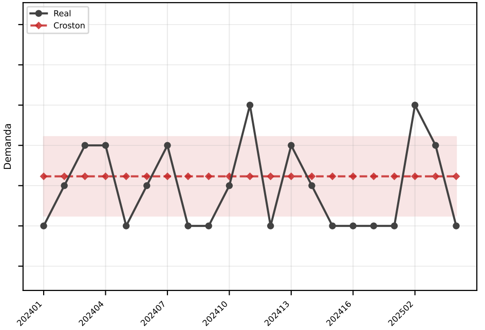
Croston MAE=1.0
