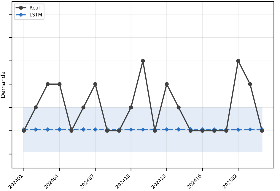
LSTM MAE=1.0
