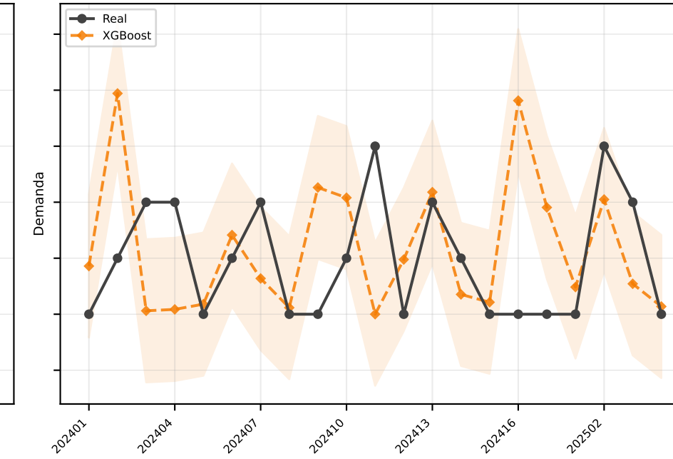
XGBoost MAE=1.3
