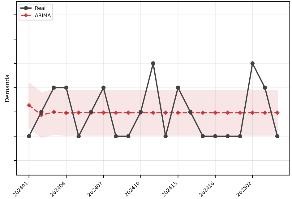
ARIMA MAE=0.9
