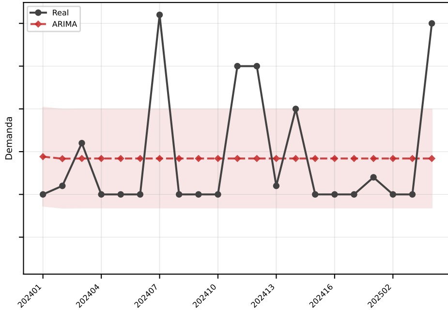
ARIMA MAE=5.8
