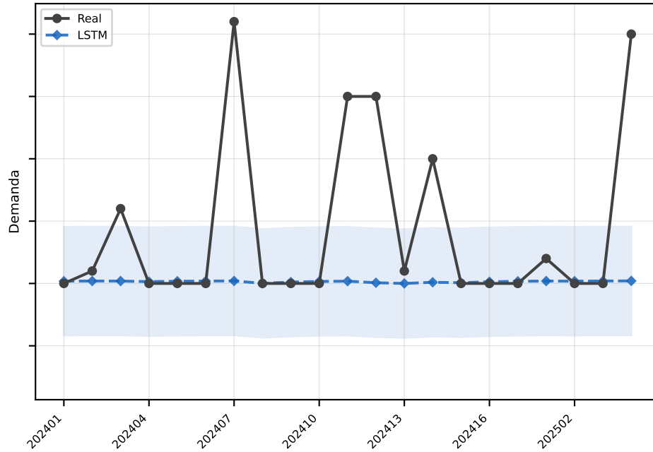
LSTM MAE=4.4
