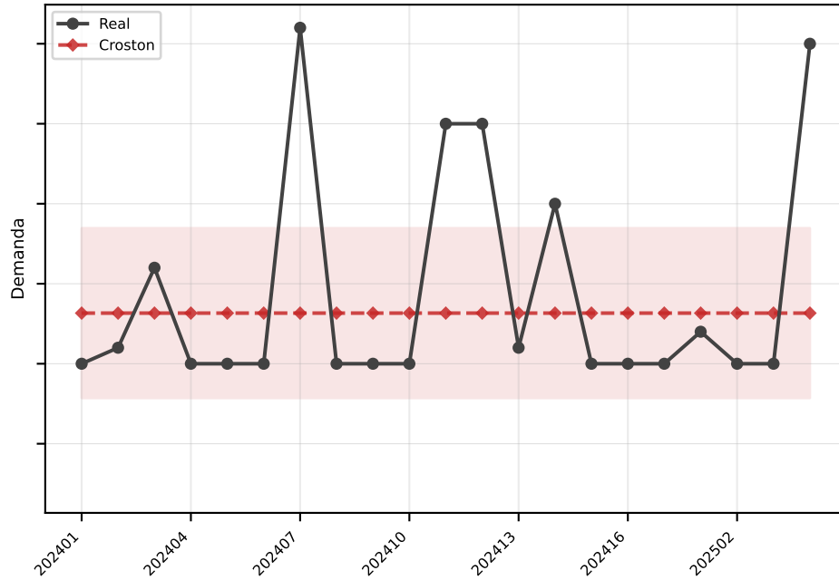
Croston MAE=5.3
