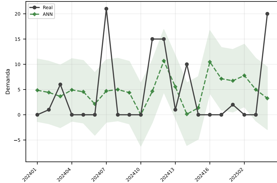
ANN MAE=6.2
