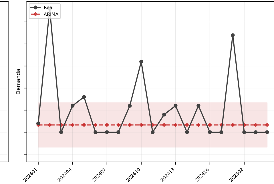
ARIMA MAE=2.5
