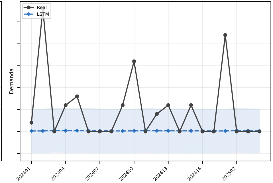
LSTM MAE=2.5
