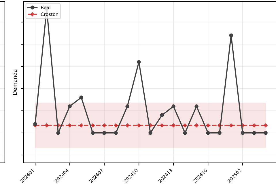
Croston MAE=2.5
