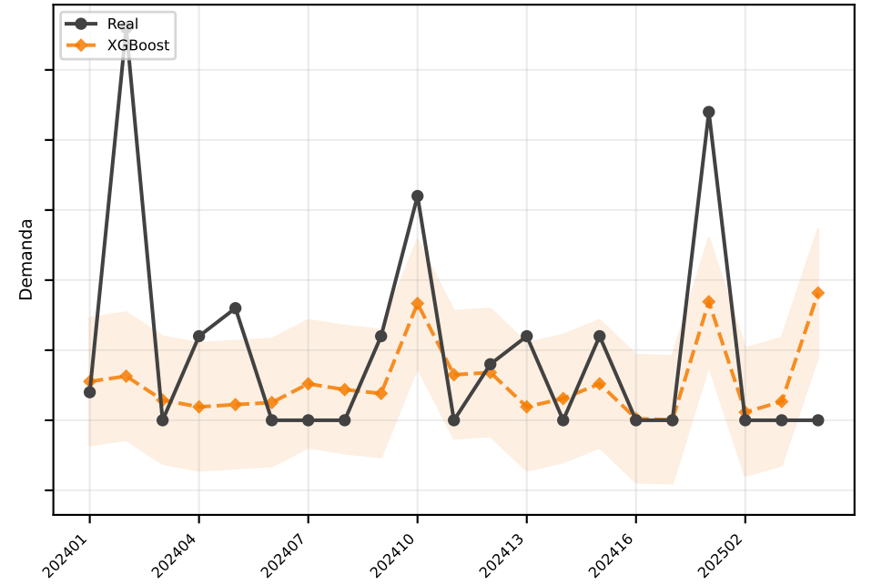
XGBoost MAE=2.3
