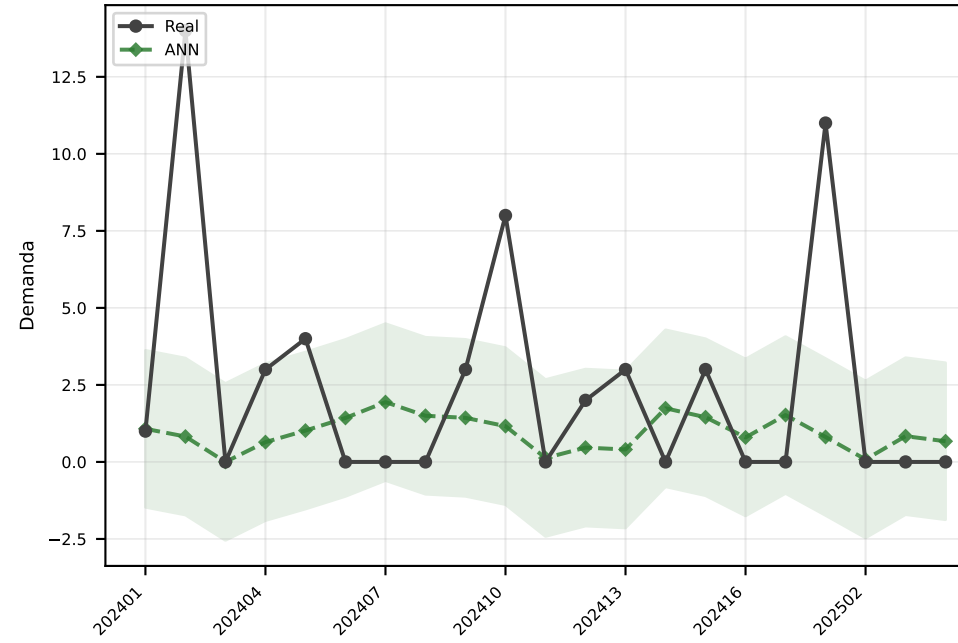
ANN MAE=2.5
