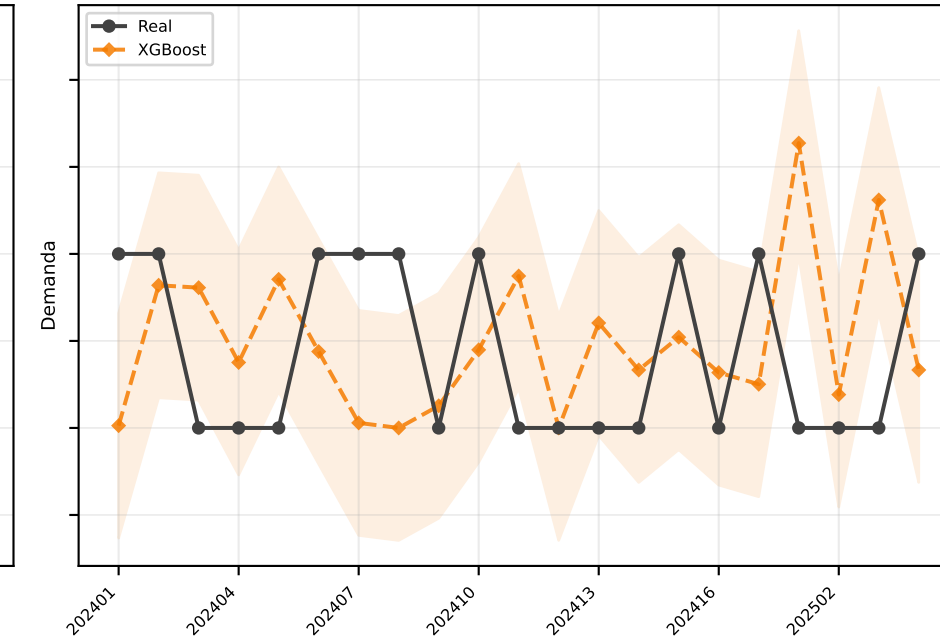
XGBoost MAE=0.6
