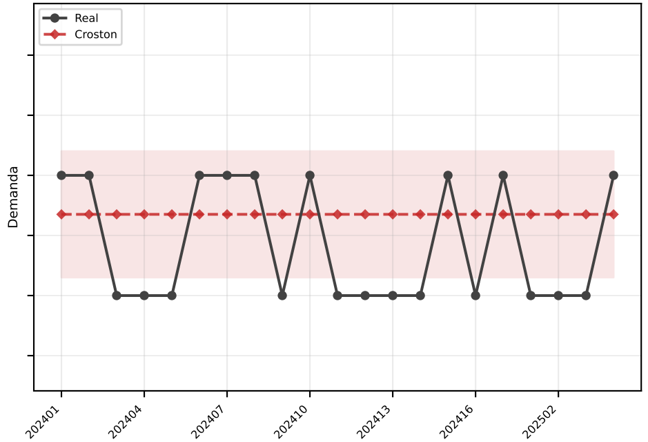
Croston MAE=0.5
