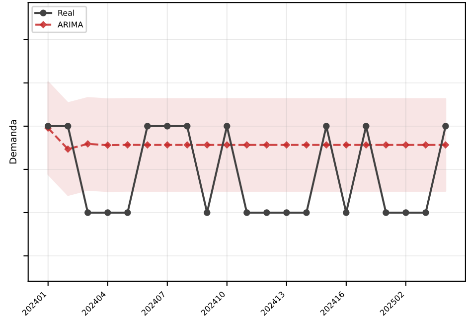
ARIMA MAE=0.5
