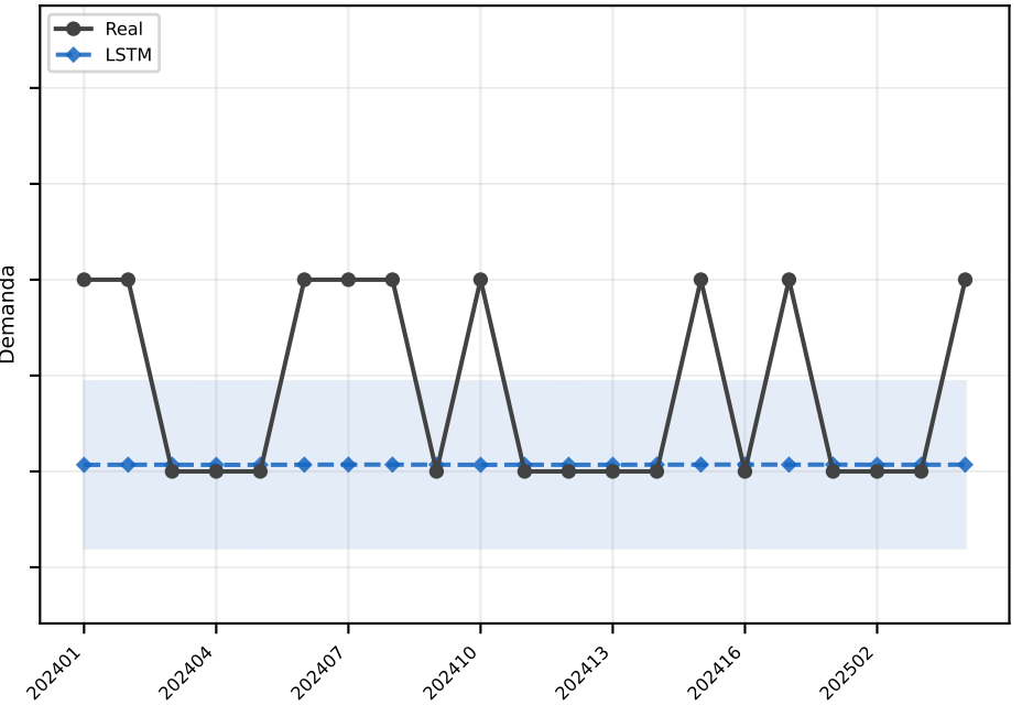
LSTM MAE=0.4
