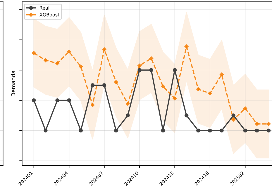
XGBoost MAE=2.3
