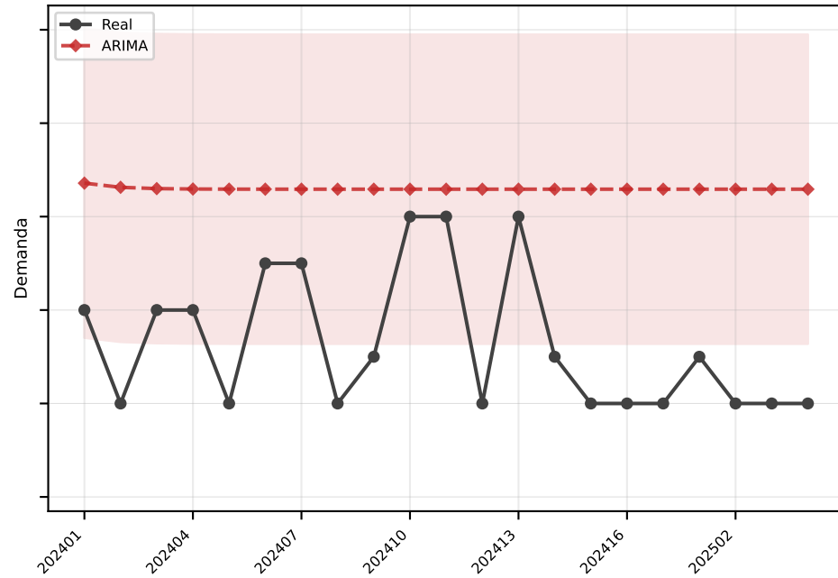
ARIMA MAE=3.3
