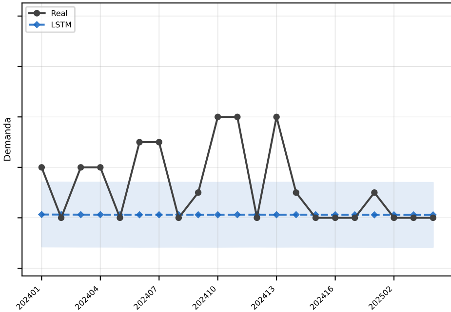
LSTM MAE=1.3
