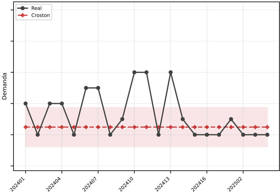
Croston MAE=1.3
