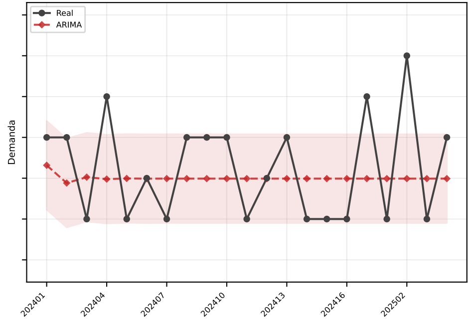
ARIMA MAE=1.1
