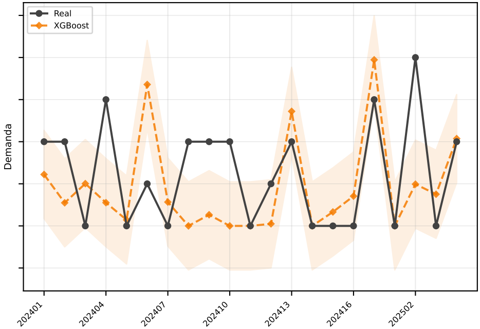
XGBoost MAE=1.0
