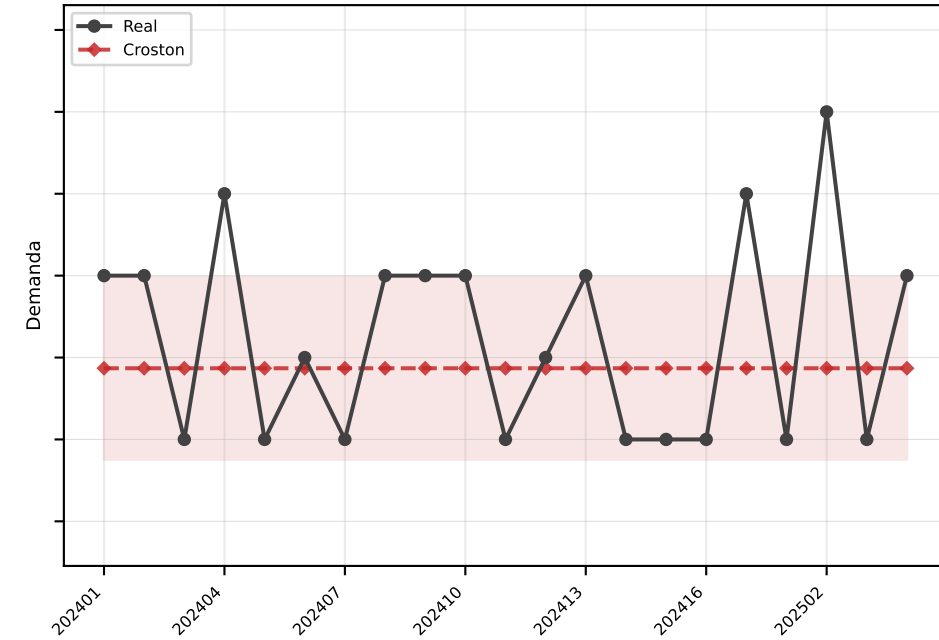
Croston MAE=1.1
