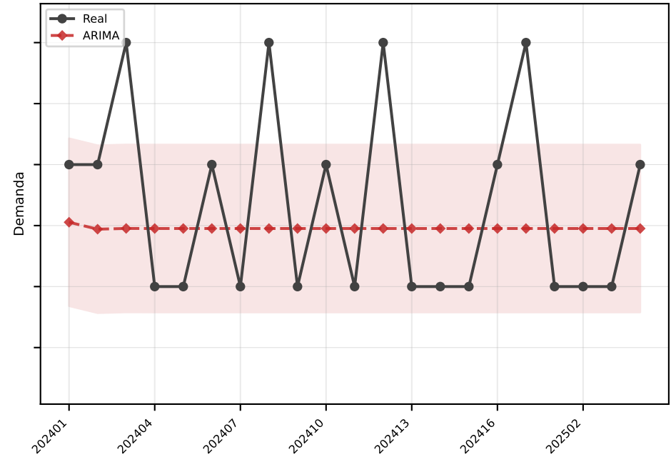
ARIMA MAE=0.7
