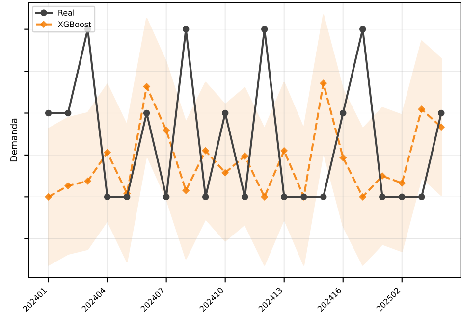
XGBoost MAE=0.8
