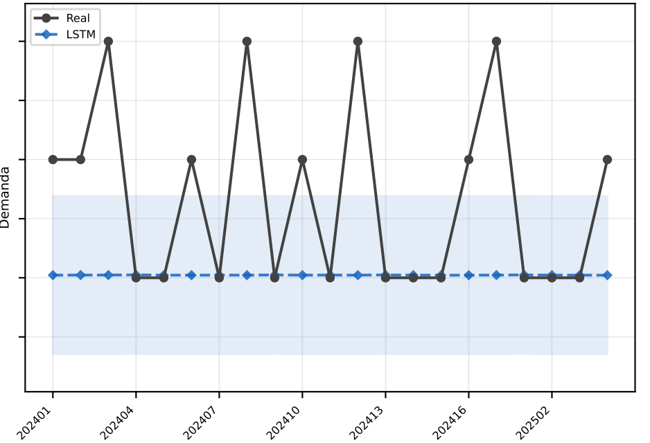
LSTM MAE=0.7
