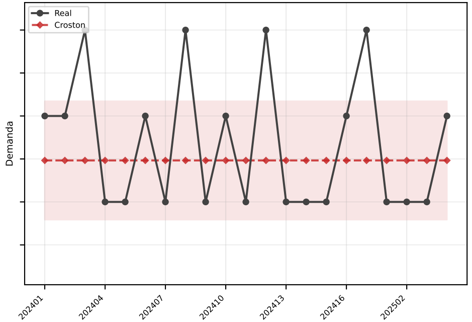
Croston MAE=0.7
