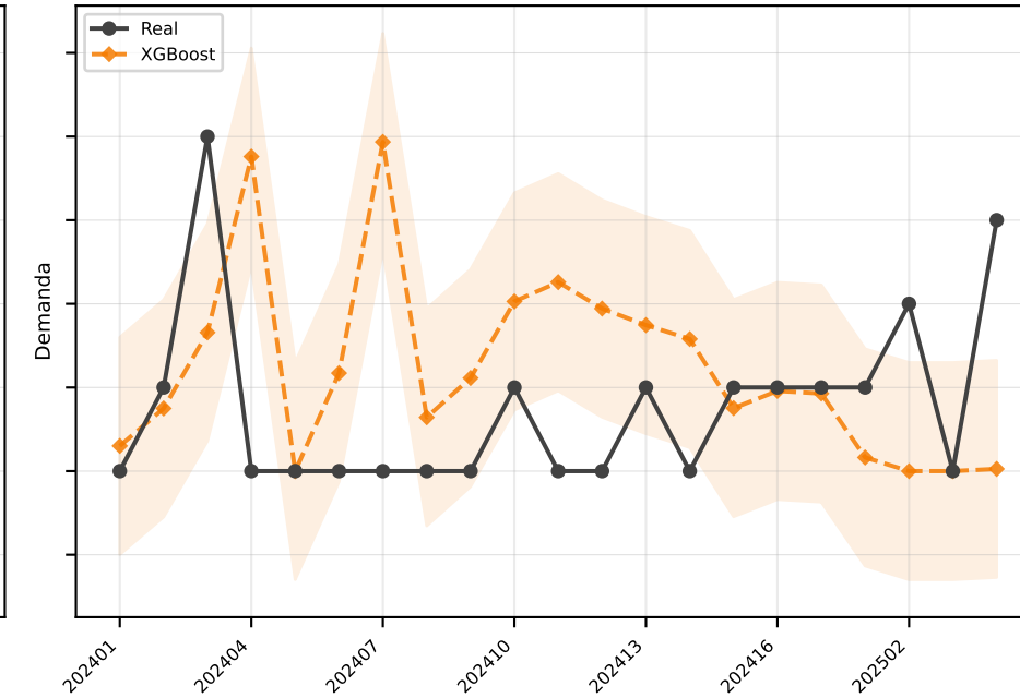
XGBoost MAE=1.3
