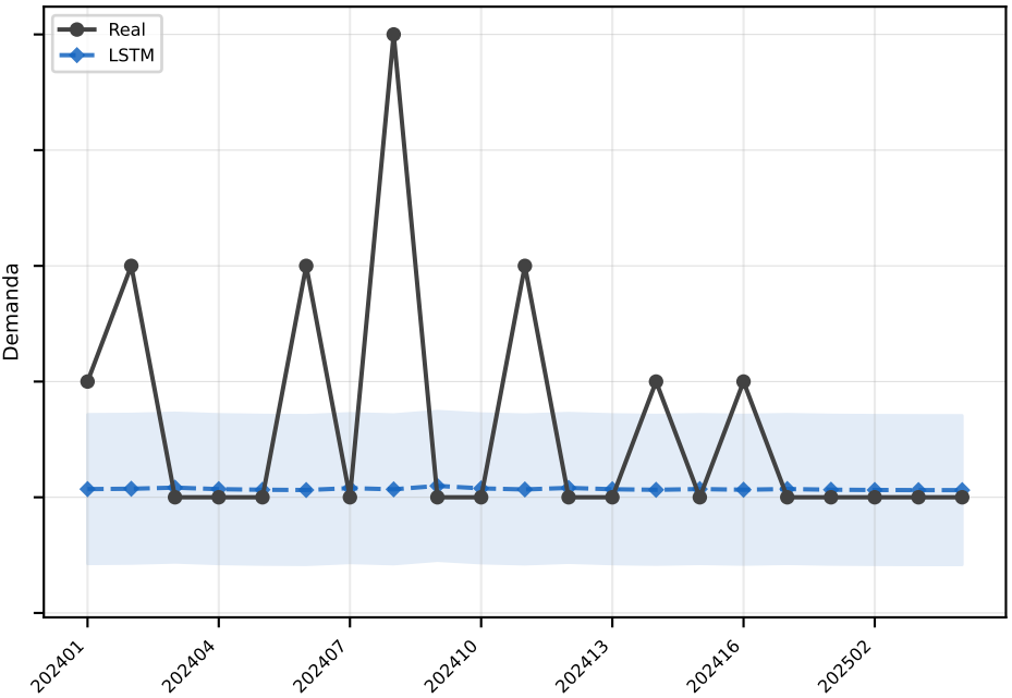
LSTM MAE=0.6
