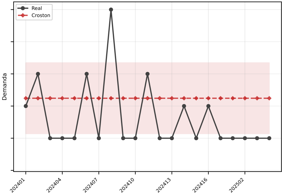
Croston MAE=1.1
