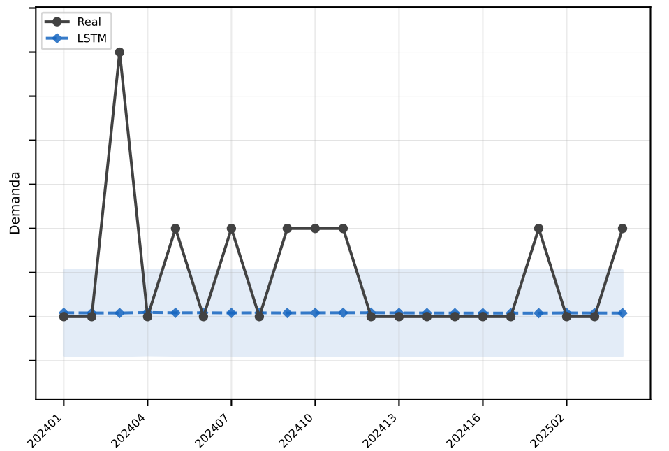
LSTM MAE=0.5
