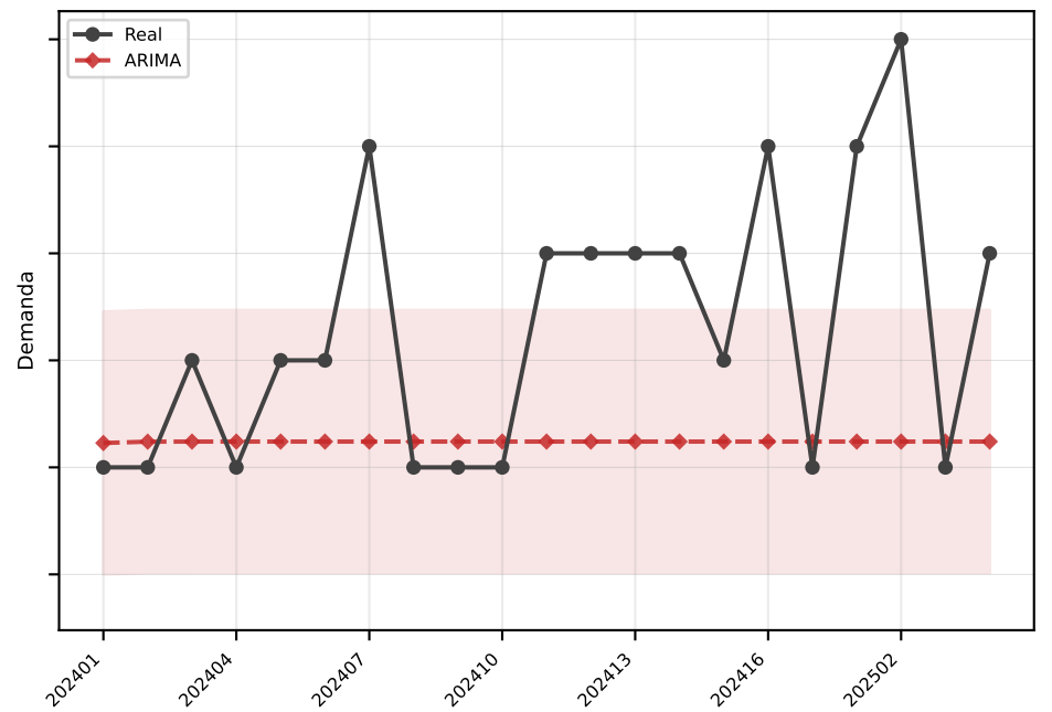
ARIMA MAE=1.2
