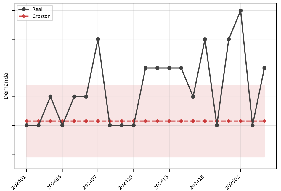
Croston MAE=1.2
