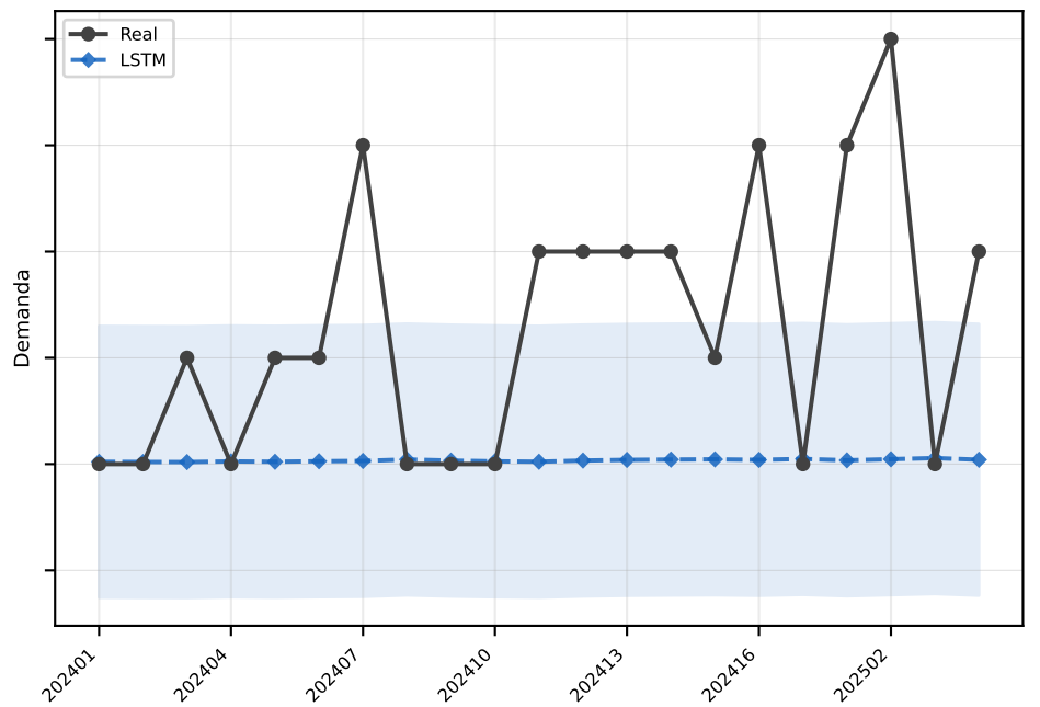
LSTM MAE=1.3
