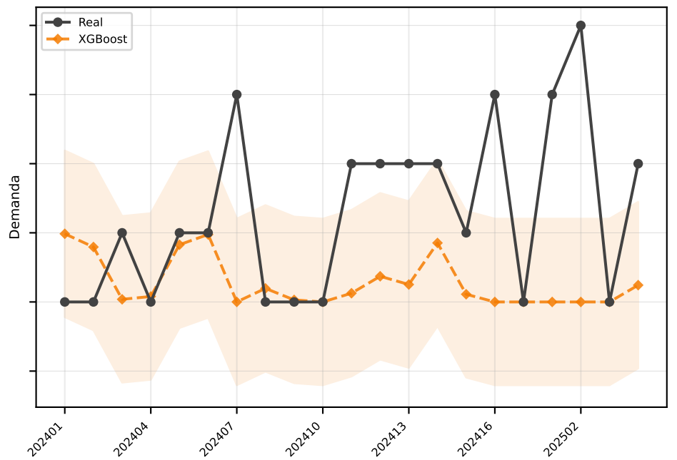
XGBoost MAE=1.2
