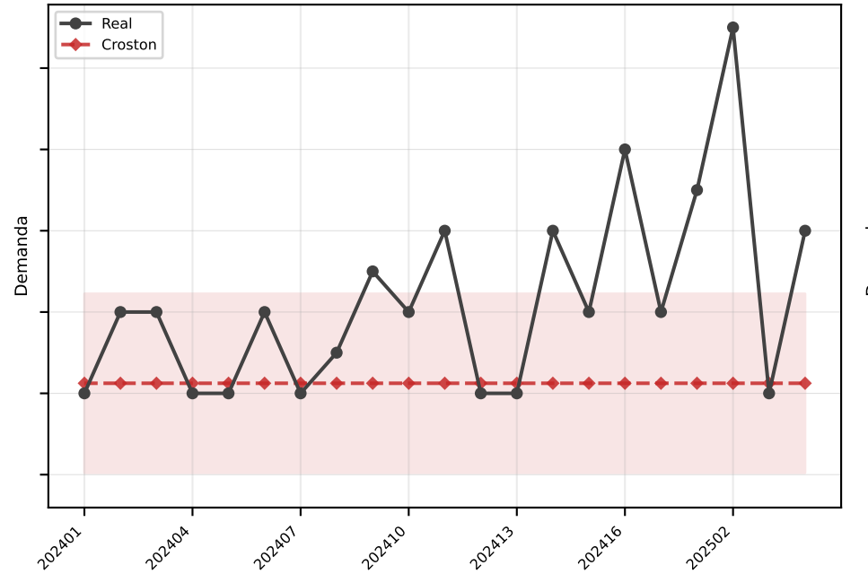
Croston MAE=2.2
