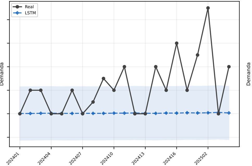
LSTM MAE=2.3
