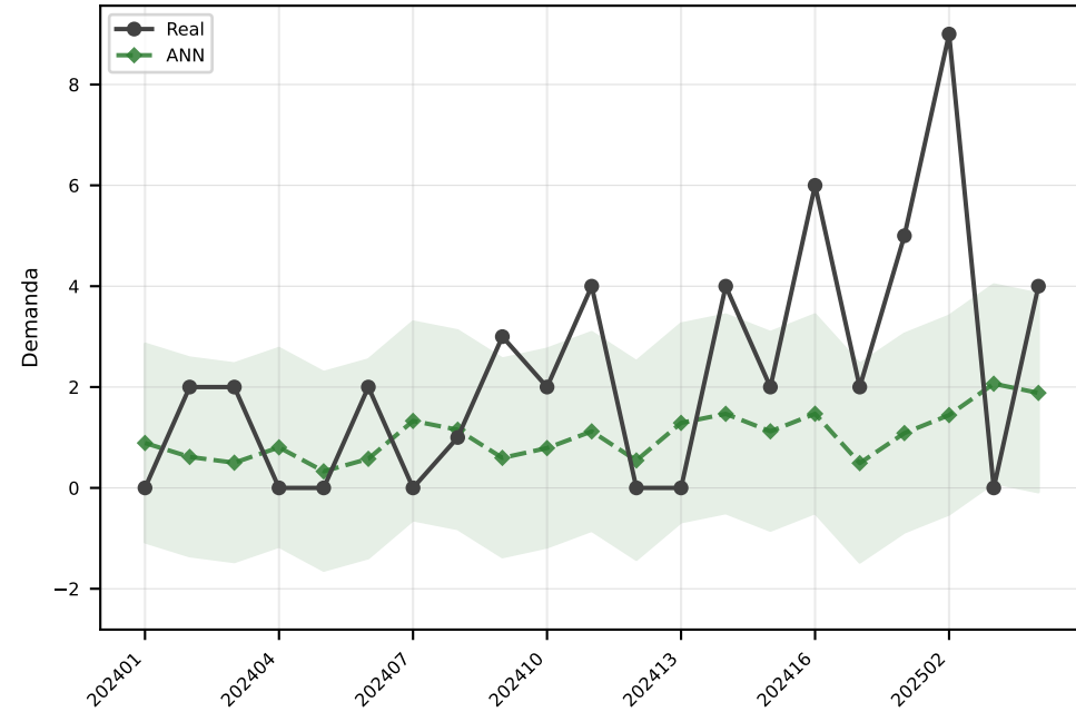
ANN MAE=2.0
