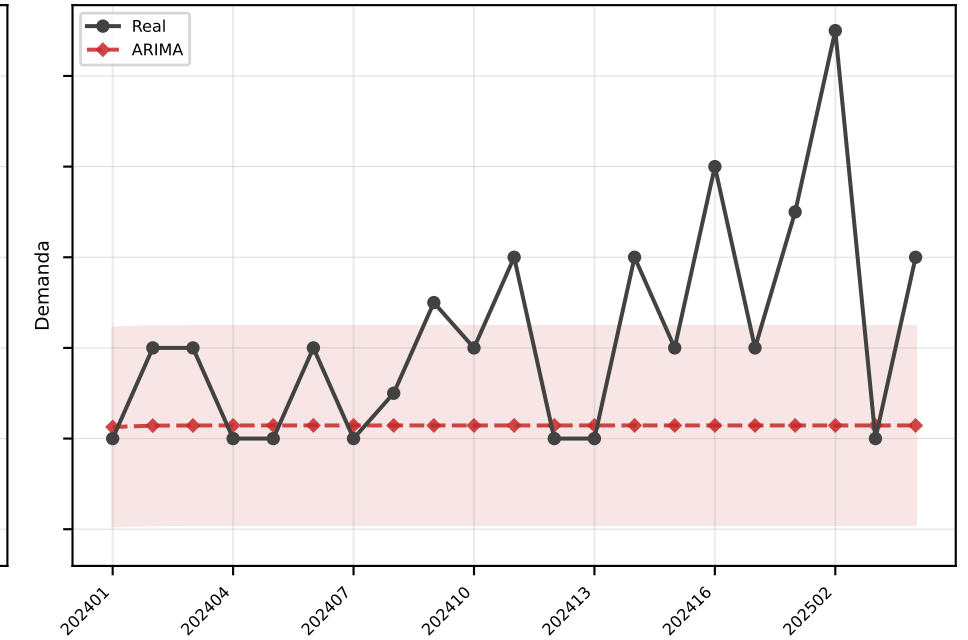
ARIMA MAE=2.2
