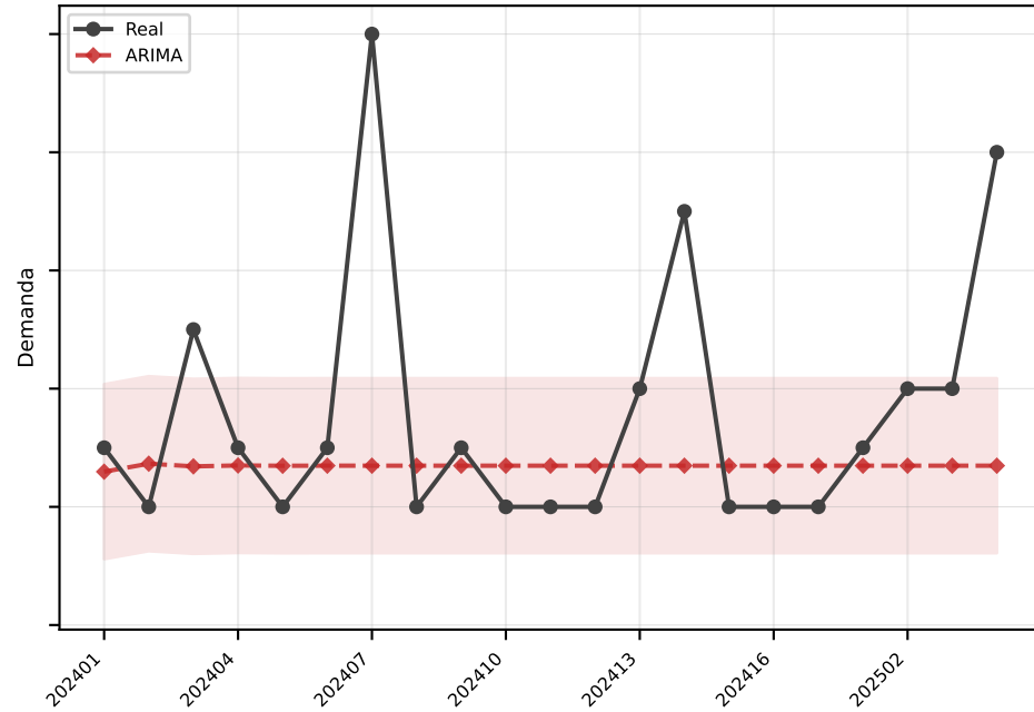
ARIMA MAE=1.5
