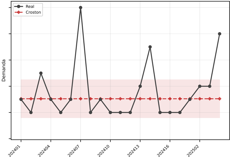
Croston MAE=1.4
