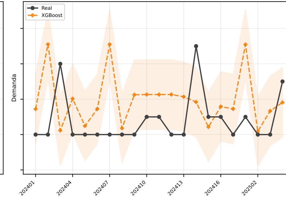
XGBoost MAE=2.0
