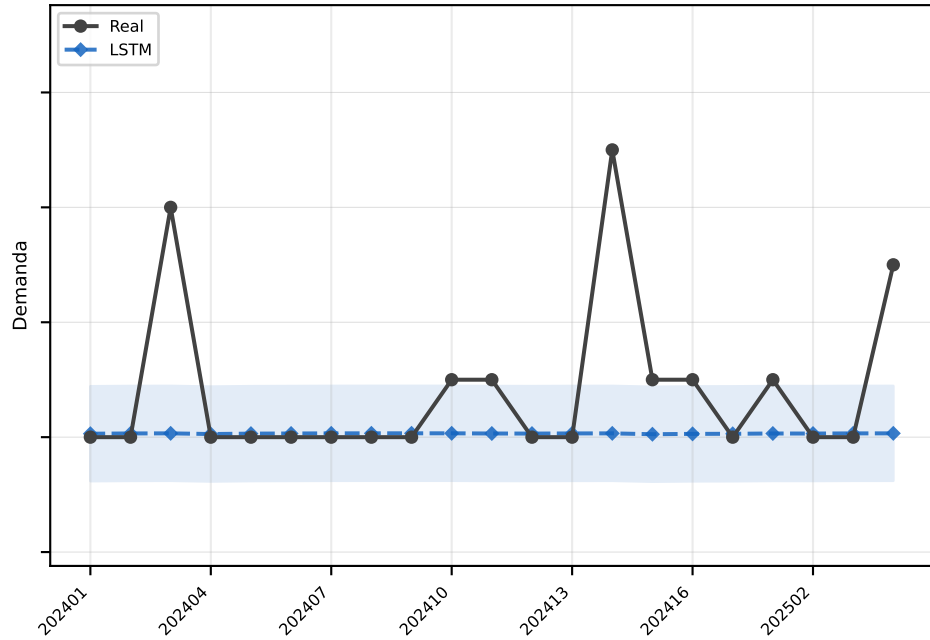
LSTM MAE=0.8
