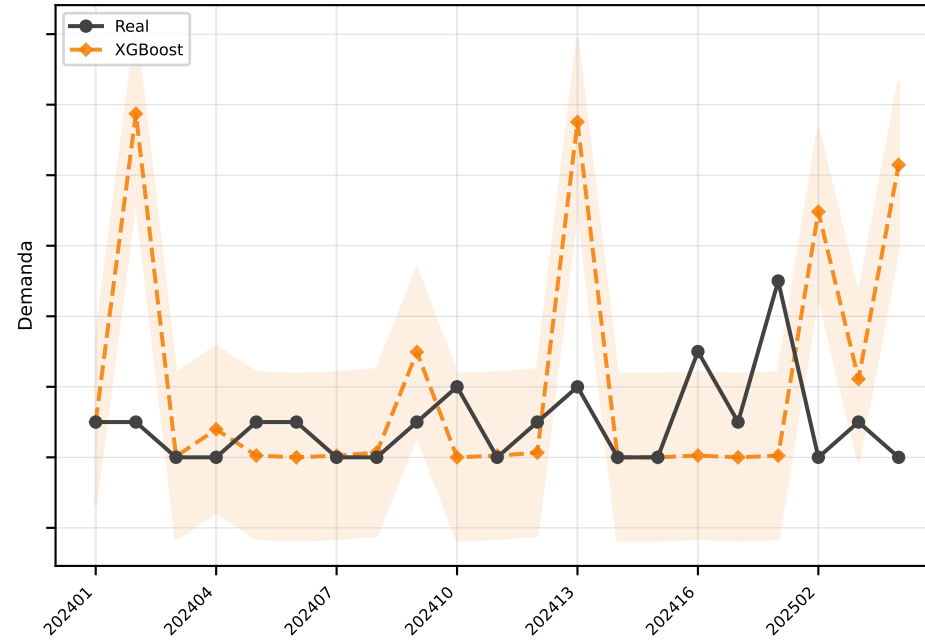
XGBoost MAE=2.4
