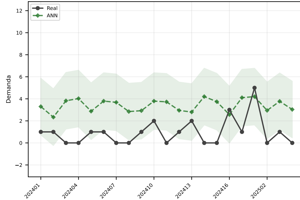
ANN MAE=2.6
