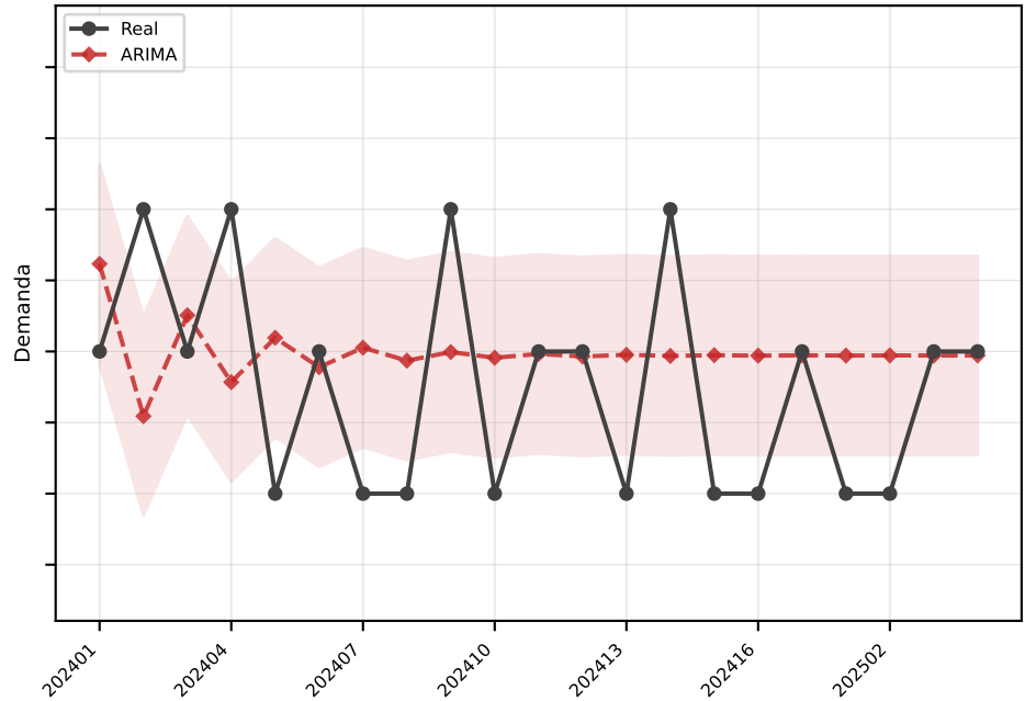
ARIMA MAE=0.7
