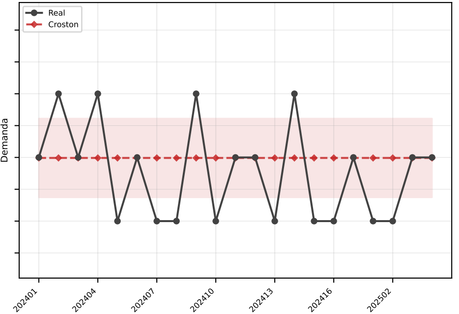
Croston MAE=0.6
