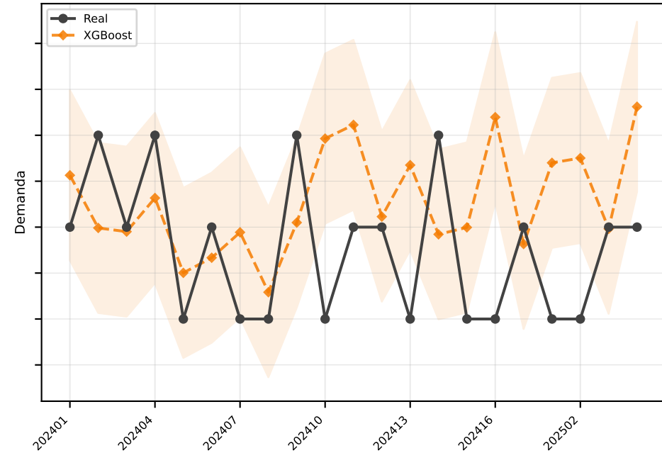
XGBoost MAE=0.9
