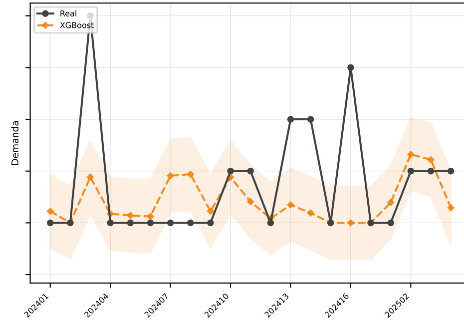
XGBoost MAE=0.7
