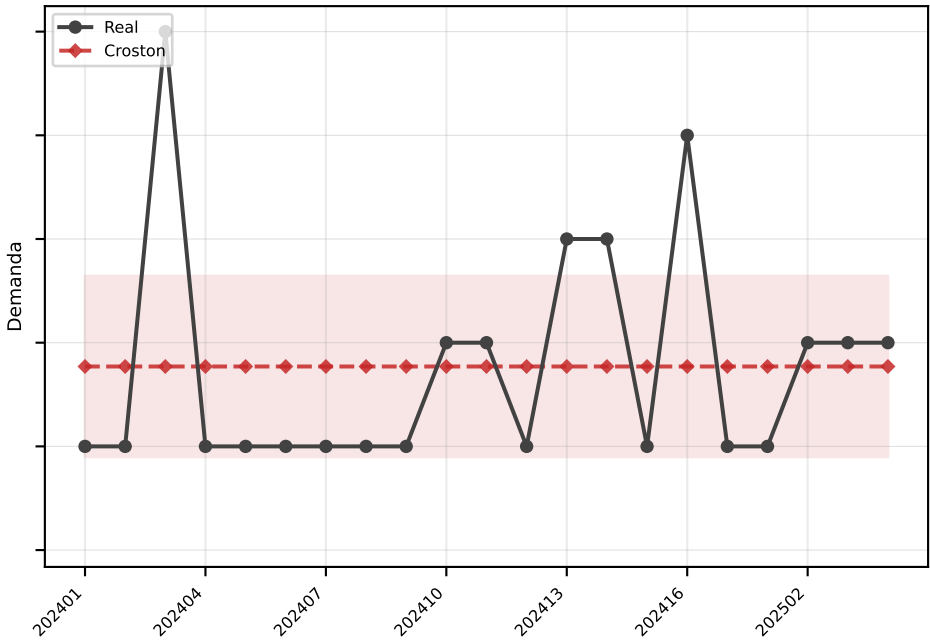
Croston MAE=0.9
