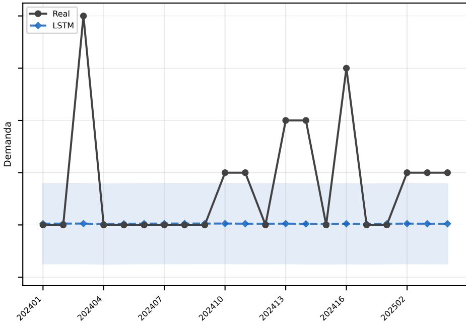
LSTM MAE=0.8
