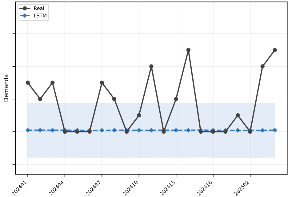
LSTM MAE=1.7
