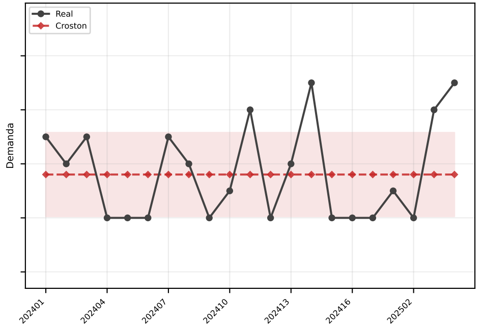
Croston MAE=1.6
