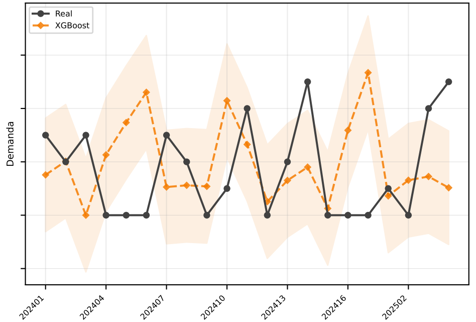
XGBoost MAE=2.1
