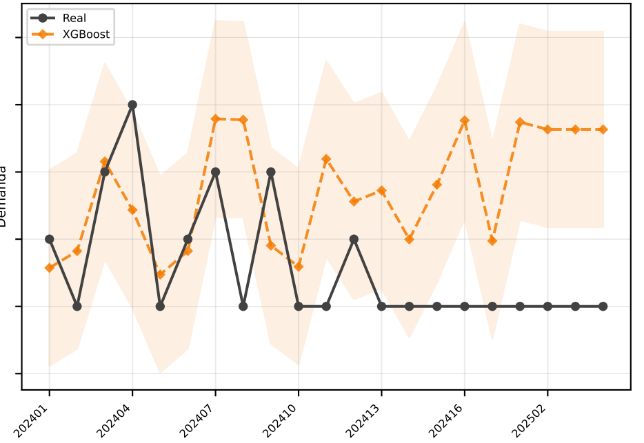
XGBoost MAE=1.5
