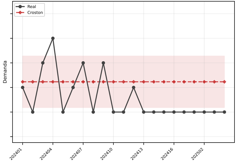
Croston MAE=1.0
