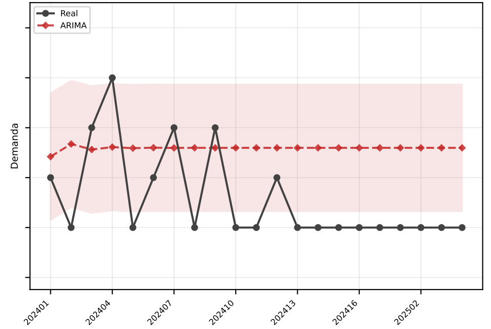
ARIMA MAE=1.3
