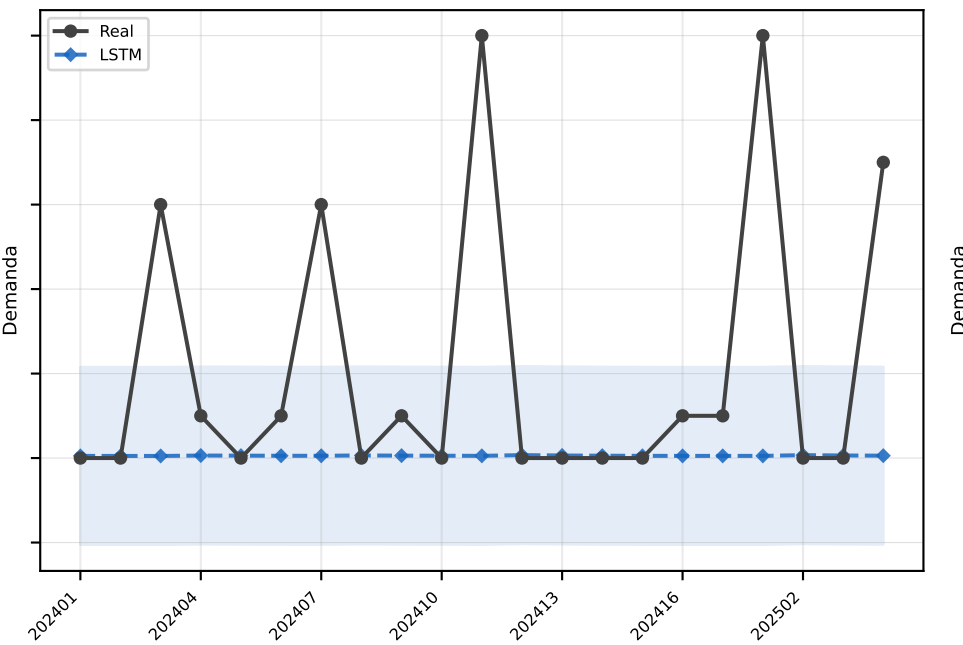
LSTM MAE=2.1
