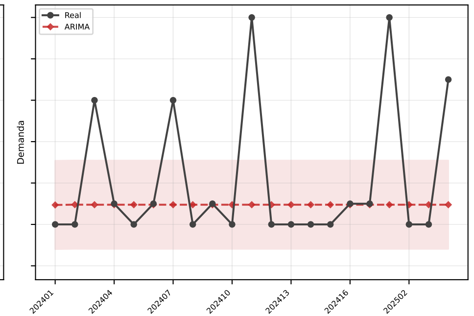
ARIMA MAE=2.1
