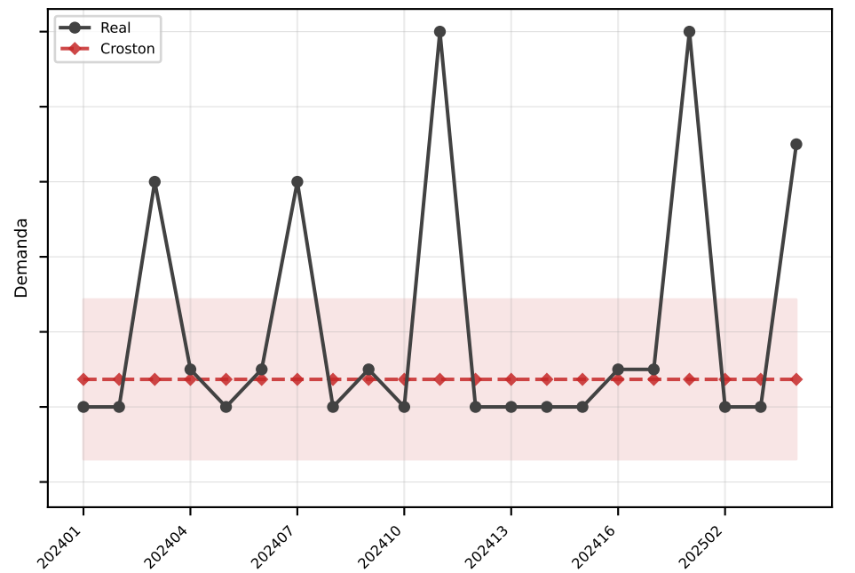
Croston MAE=2.1
