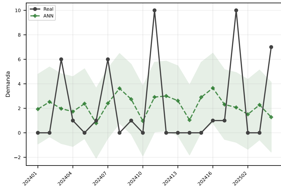
ANN MAE=2.8
