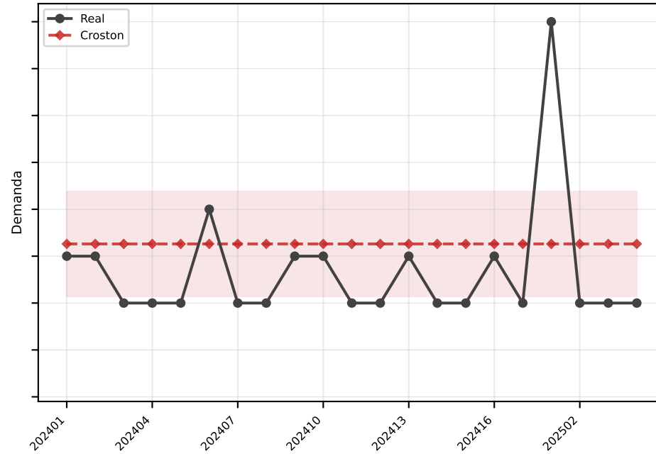
Croston MAE=1.1
