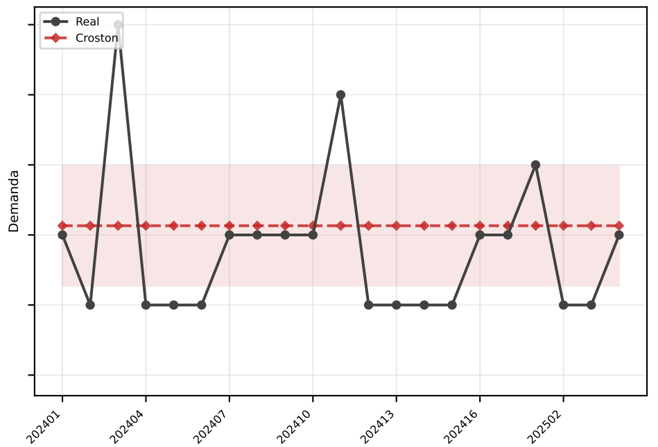
Croston MAE=0.9
