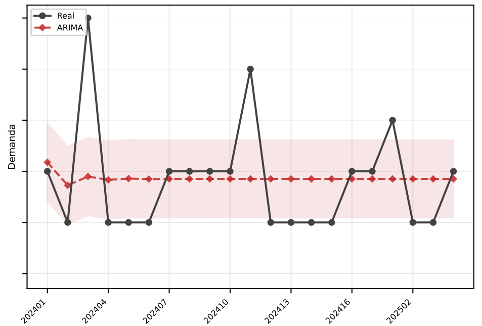
ARIMA MAE=0.8
