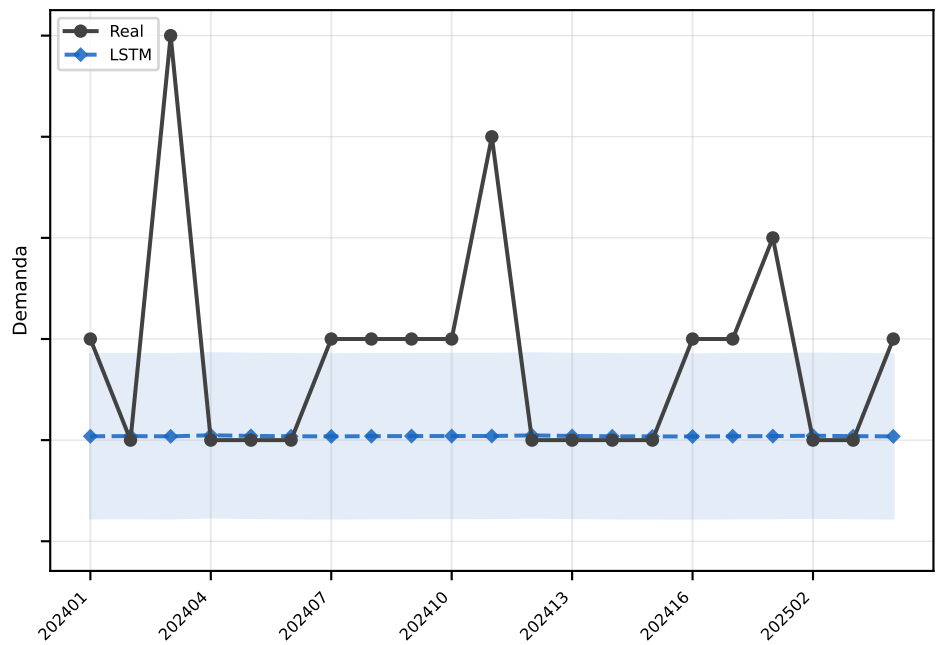
LSTM MAE=0.8
