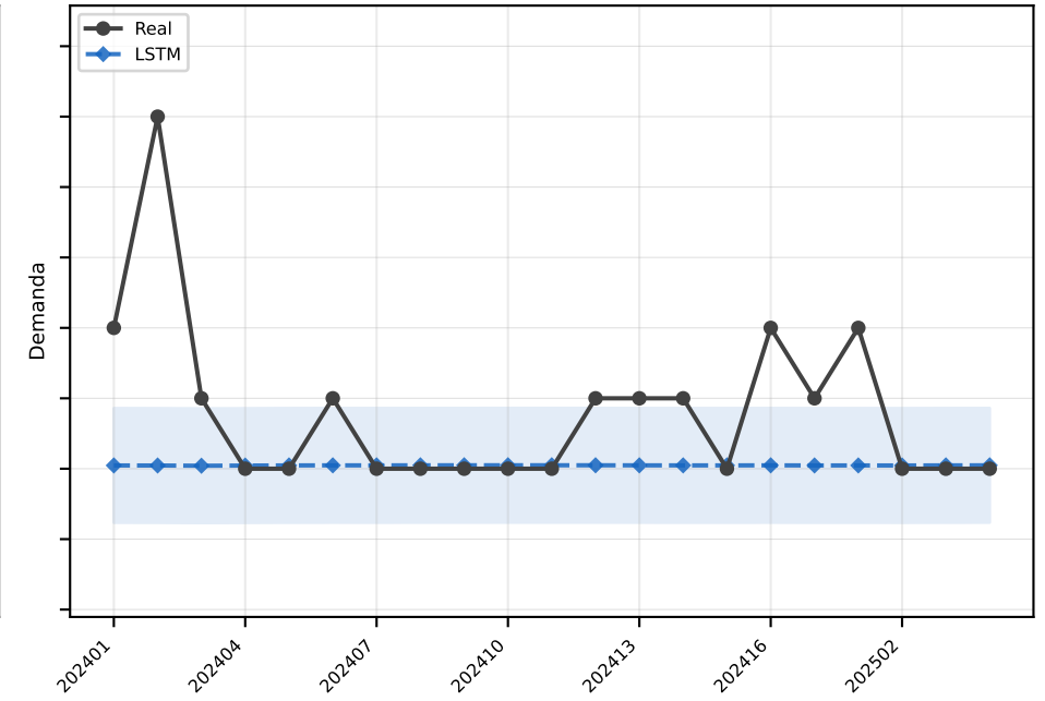
LSTM MAE=0.8
