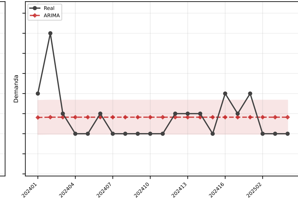
ARIMA MAE=0.8
