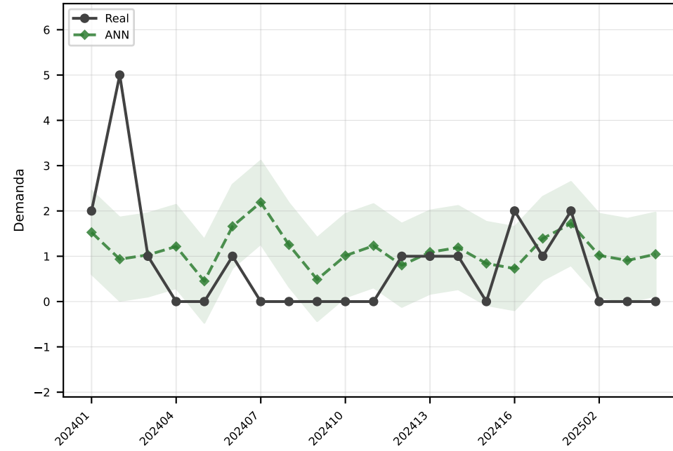
ANN MAE=0.9
