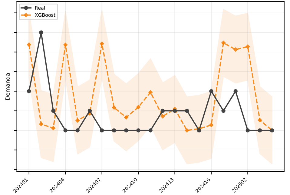
XGBoost MAE=1.7
