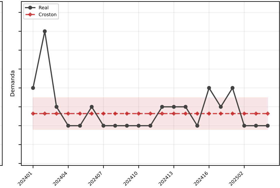
Croston MAE=0.8
