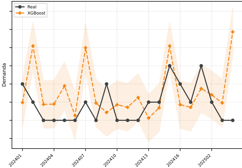
XGBoost MAE=1.3
