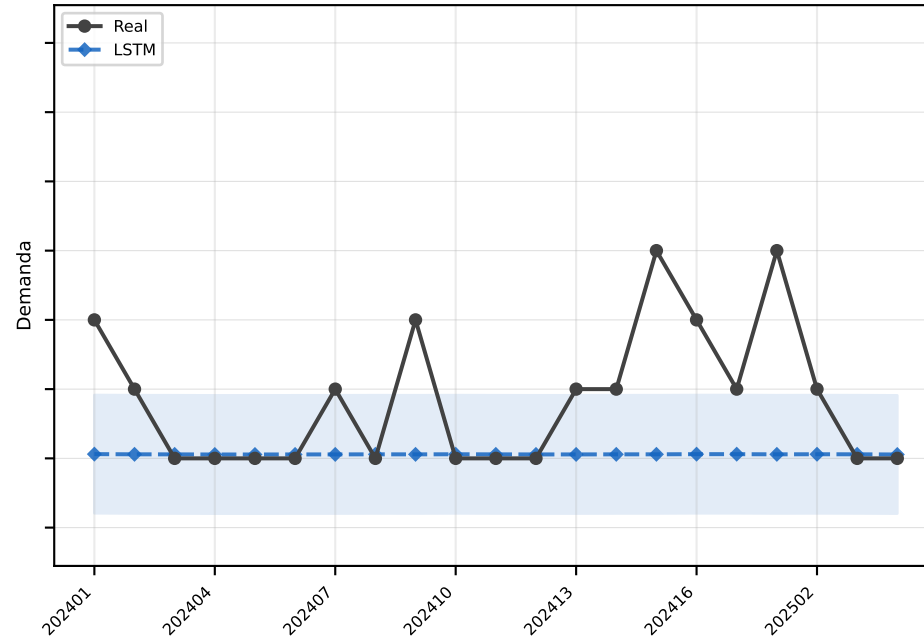
LSTM MAE=0.9
