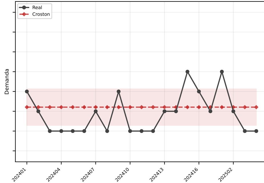
Croston MAE=0.9
