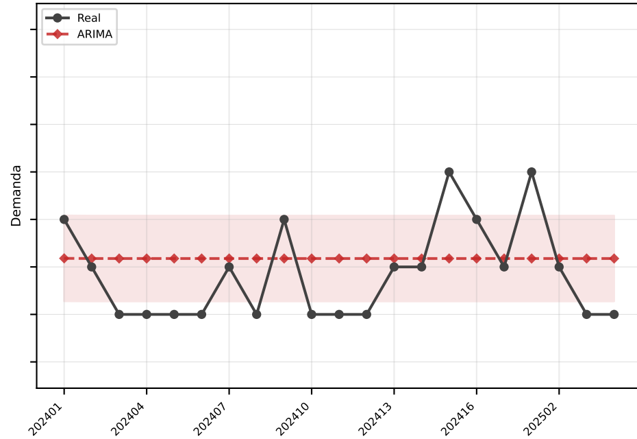
ARIMA MAE=0.9
