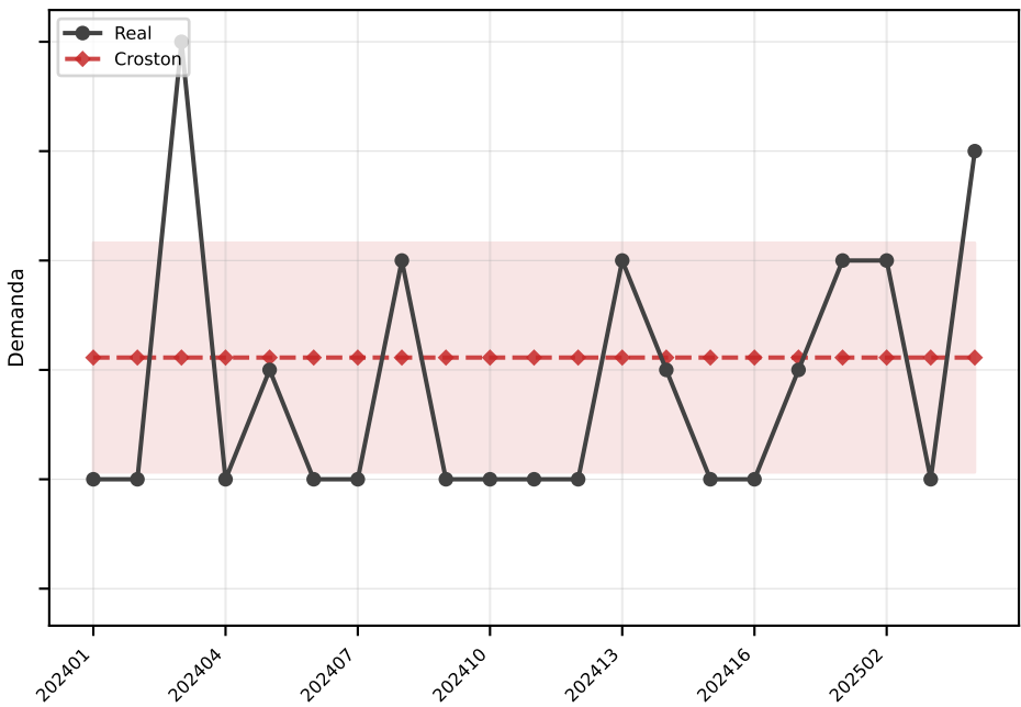
Croston MAE=1.0
