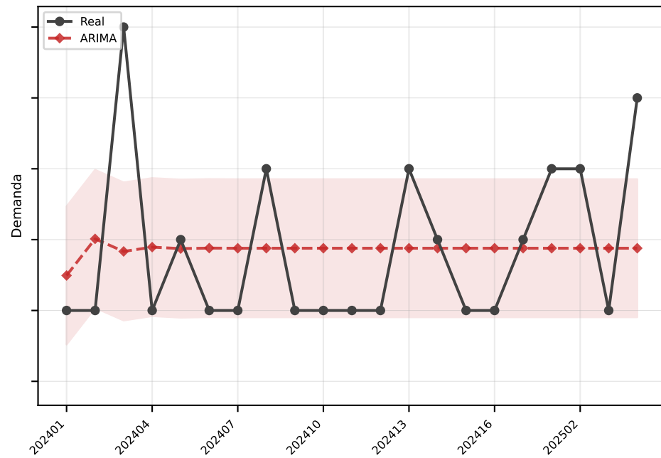
ARIMA MAE=1.0
