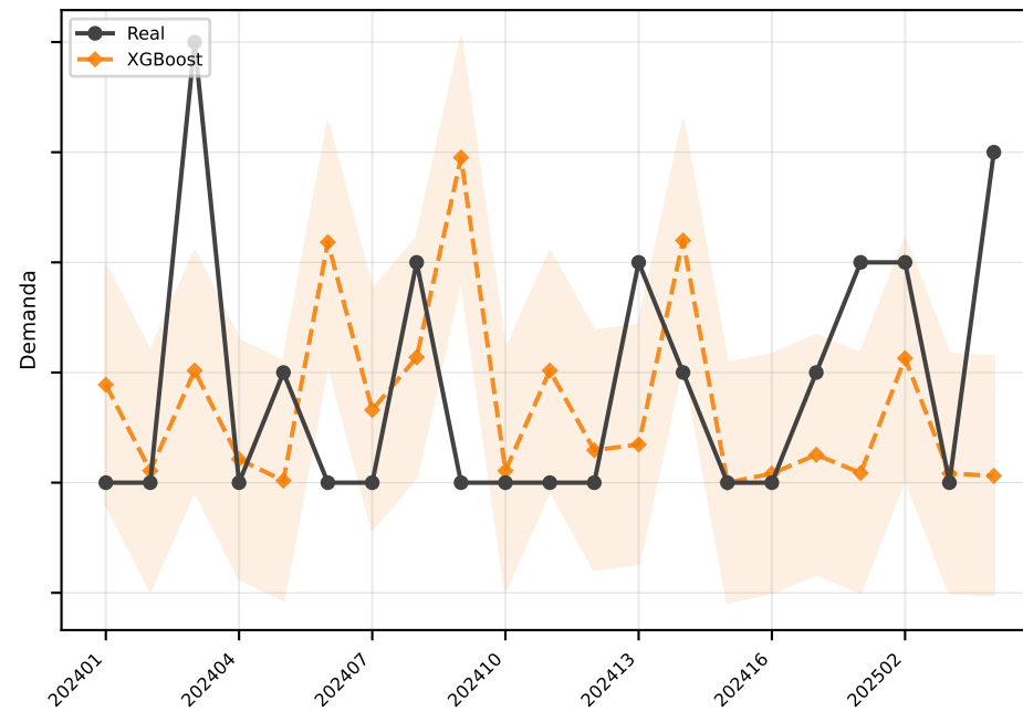
XGBoost MAE=1.1
