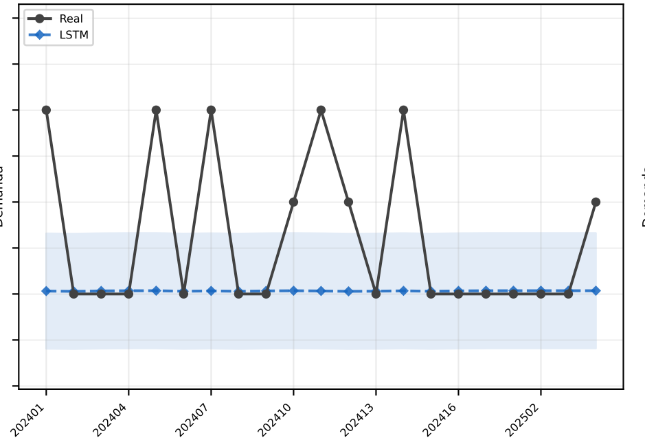
LSTM MAE=0.6
