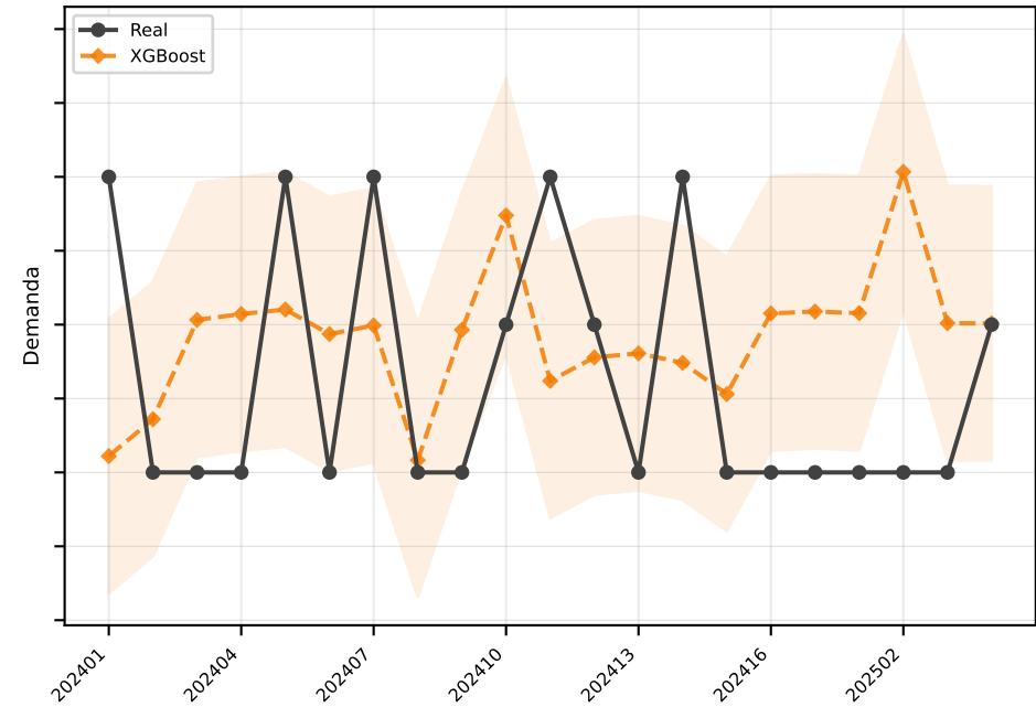
XGBoost MAE=0.9
