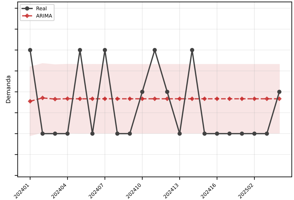
ARIMA MAE=0.8
