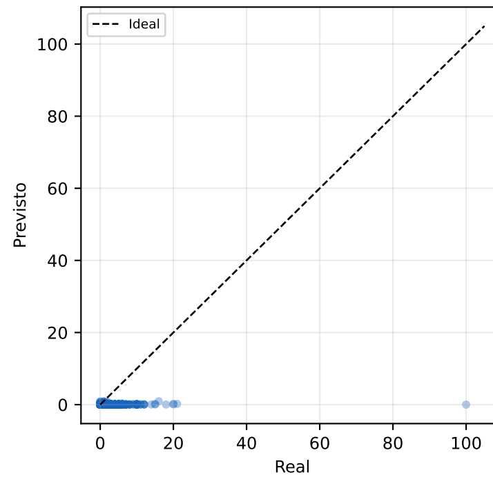
LSTM (n=3,045)
