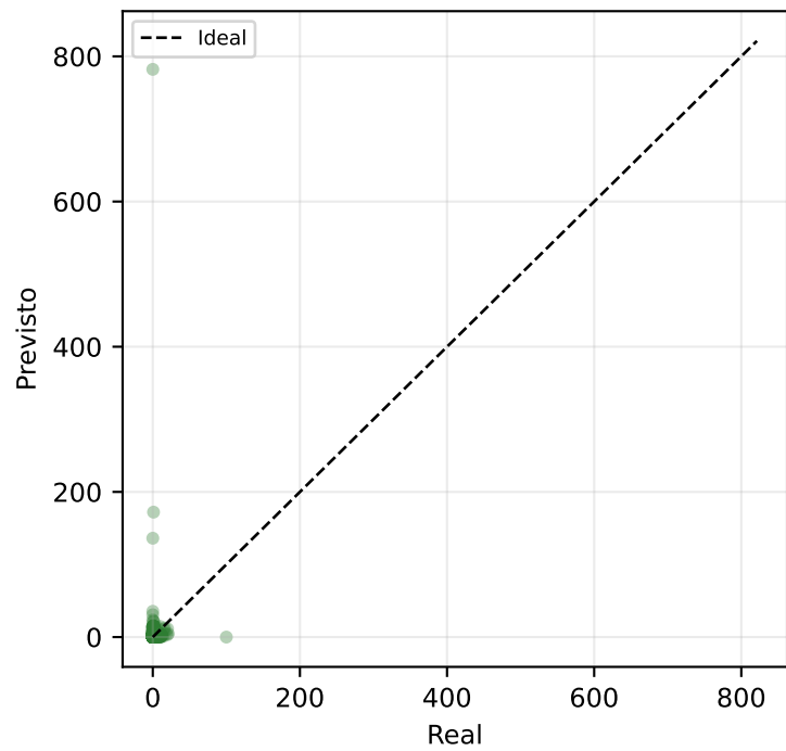
ANN (n=3,045)
