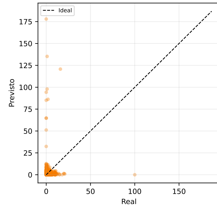
XGBoost (n=3,045)
