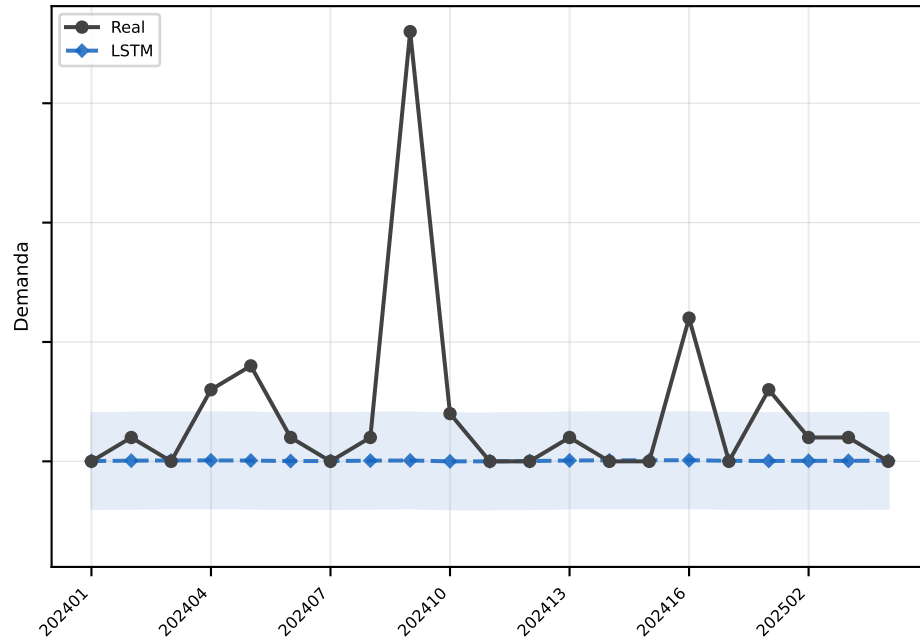
LSTM MAE=2.0
