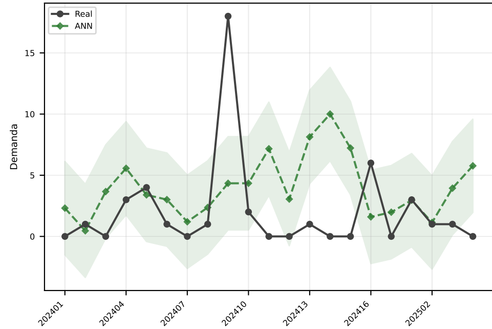
ANN MAE=3.8
