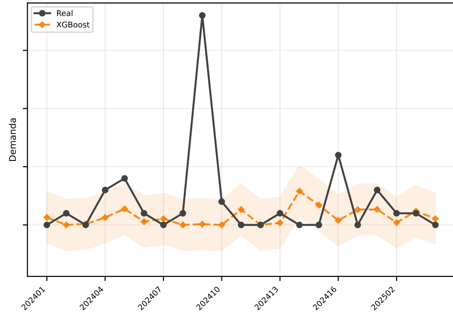
XGBoost MAE=2.2
