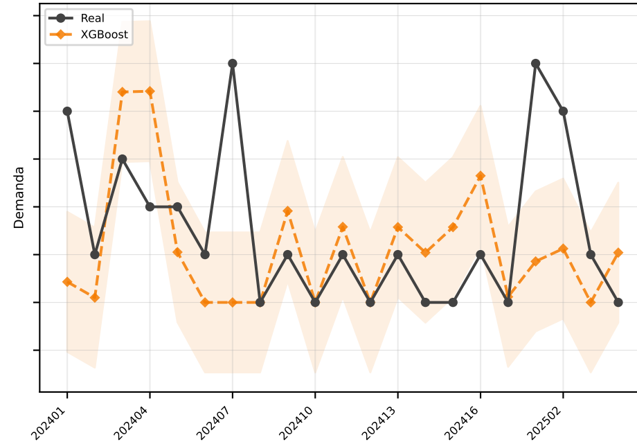
XGBoost MAE=1.5
