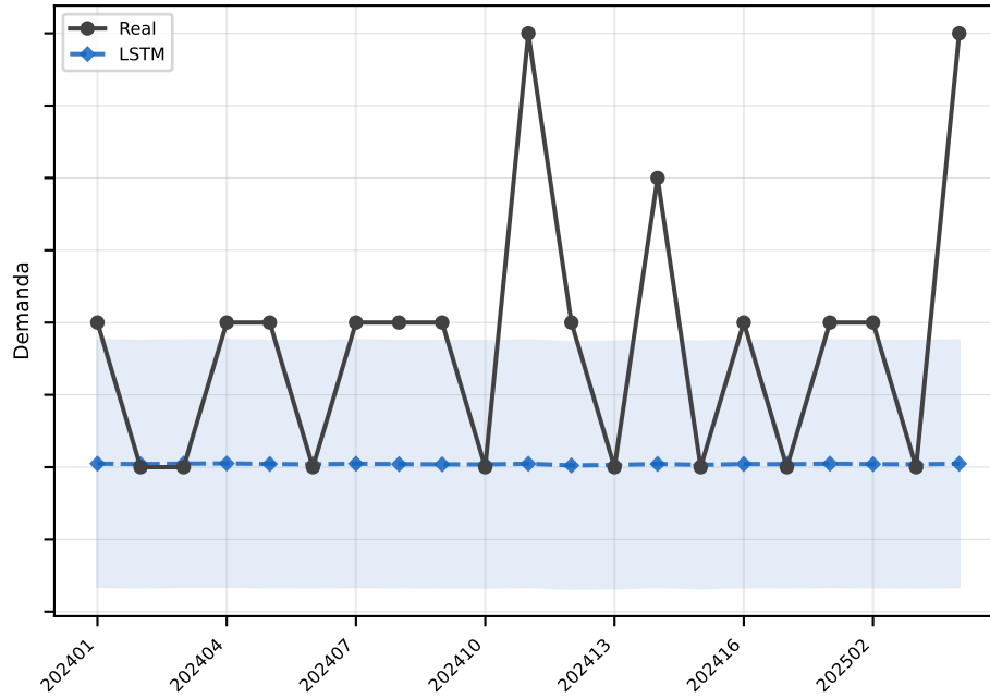
LSTM MAE=0.9
