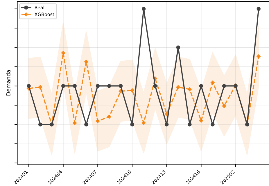
XGBoost MAE=0.8
