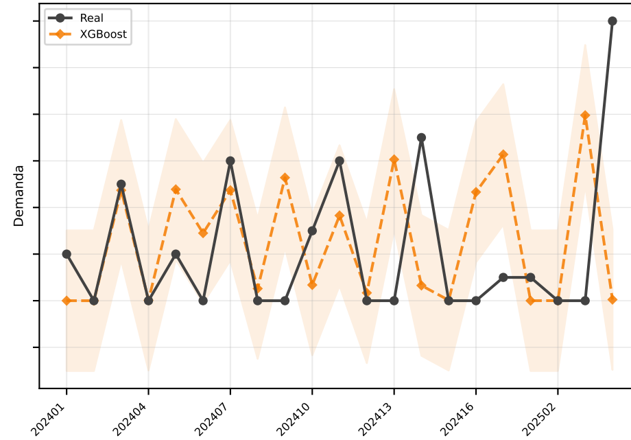
XGBoost MAE=3.0
