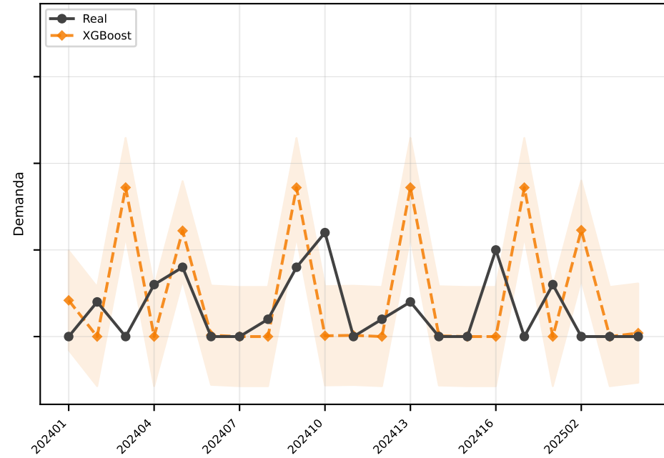
XGBoost MAE=2.9
