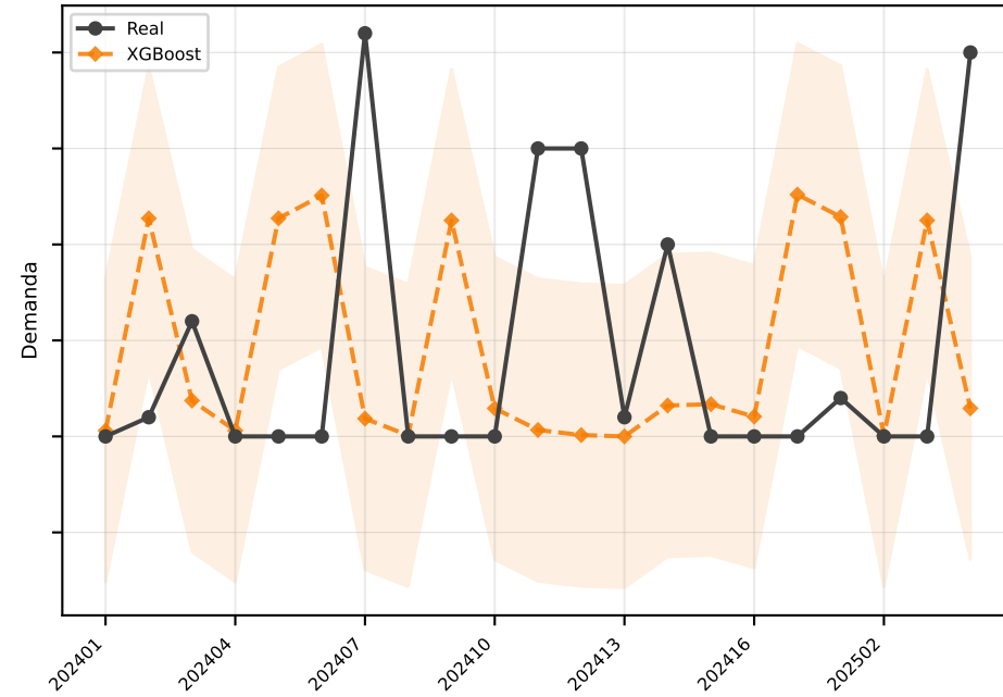
XGBoost MAE=7.9
