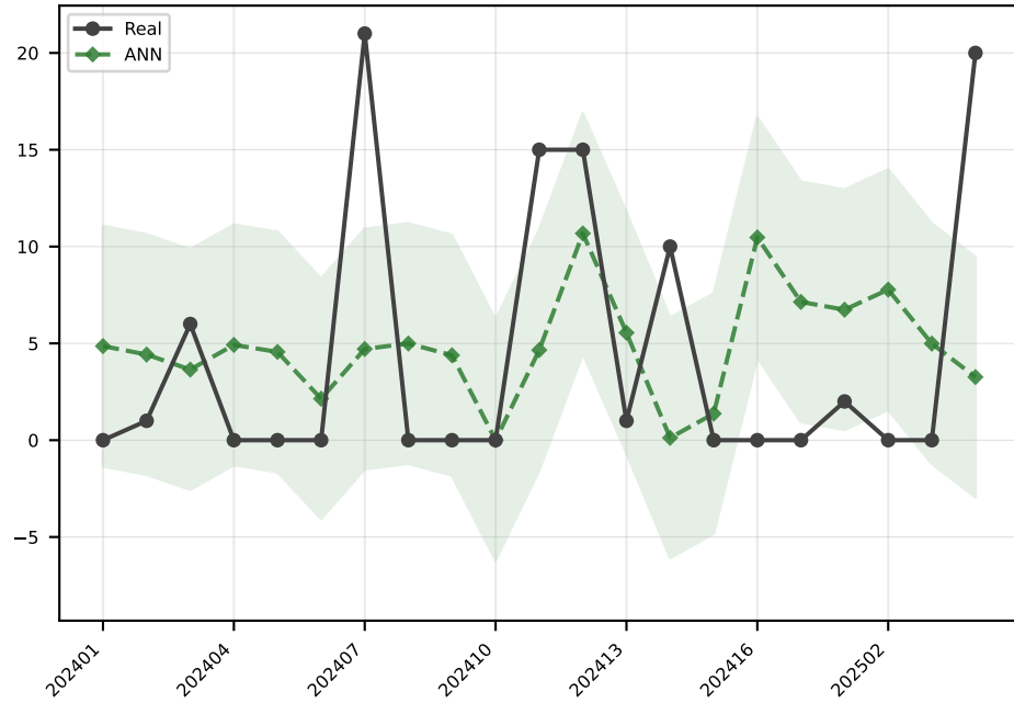
ANN MAE=6.2
