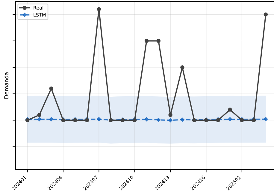
LSTM MAE=4.4
