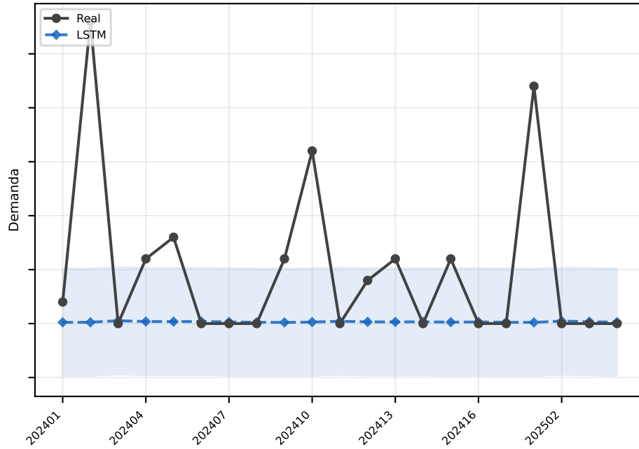
LSTM MAE=2.5
