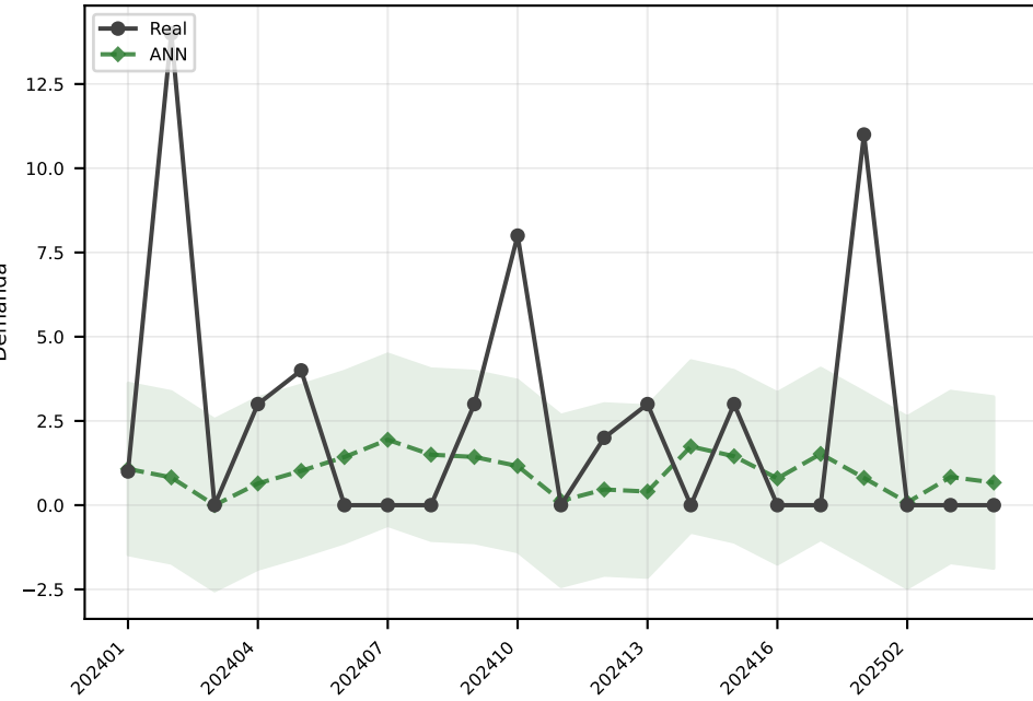
ANN MAE=2.5
