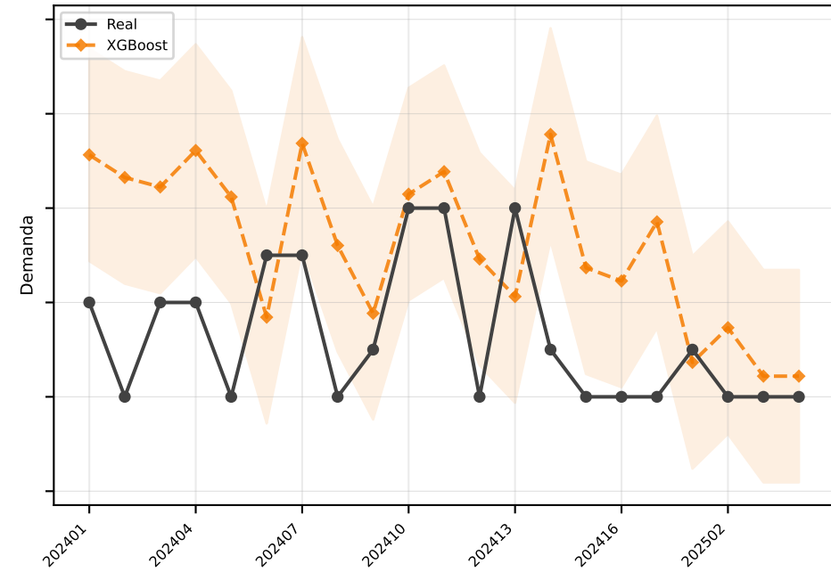
XGBoost MAE=2.3
