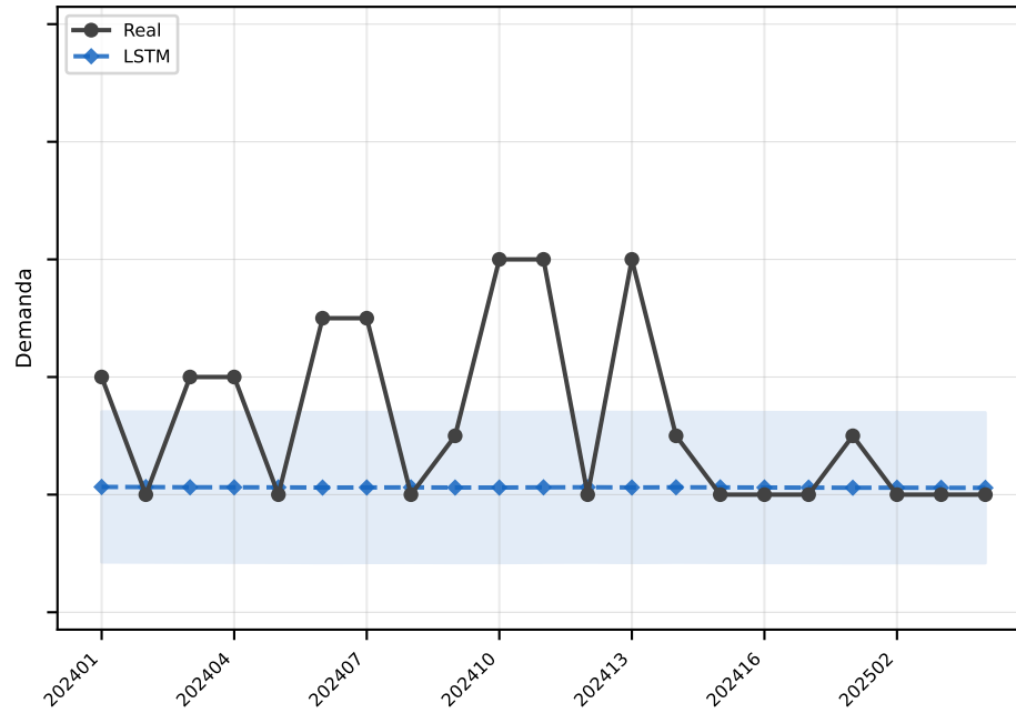
LSTM MAE=1.3
