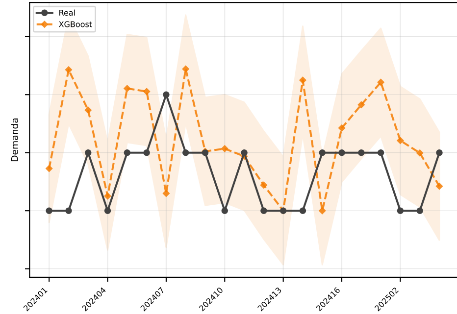
XGBoost MAE=0.9
