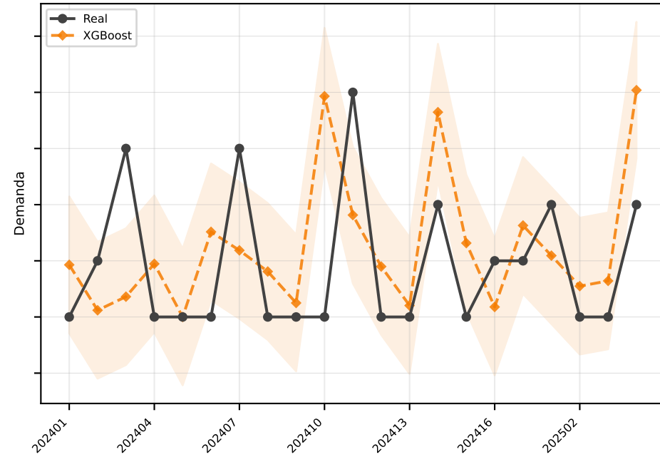
XGBoost MAE=1.2
