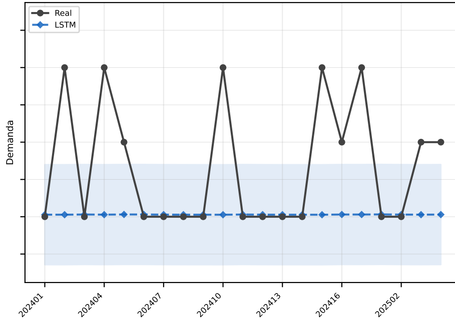
LSTM MAE=0.7
