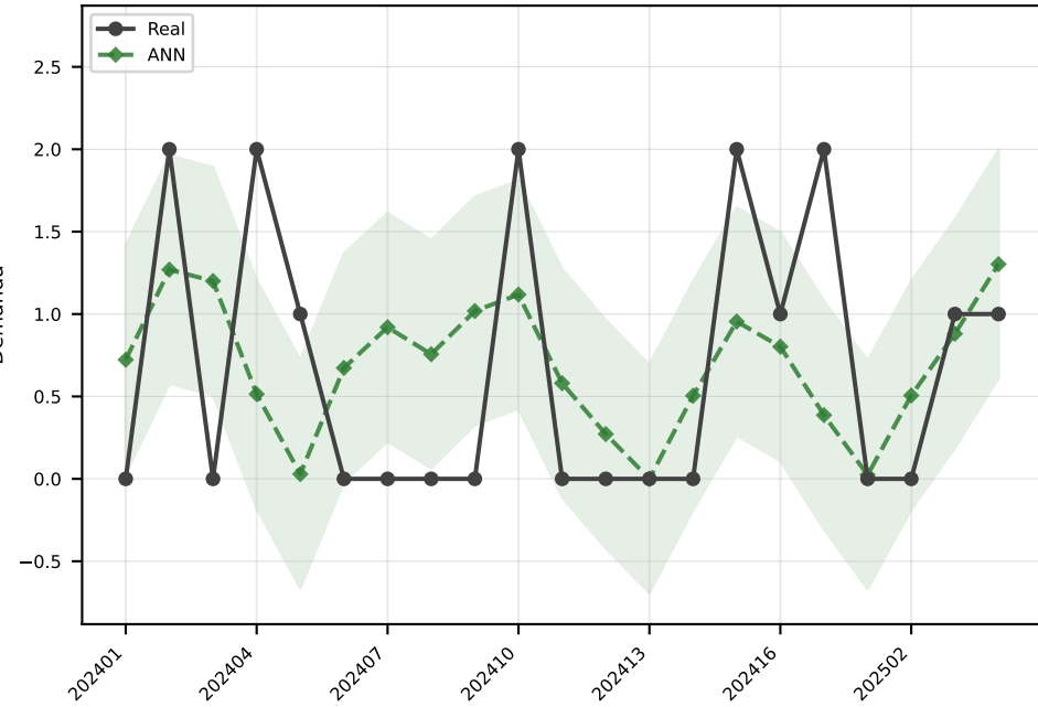
ANN MAE=0.7
