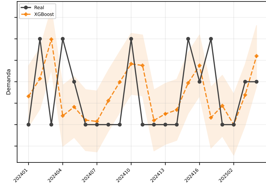
XGBoost MAE=0.7
